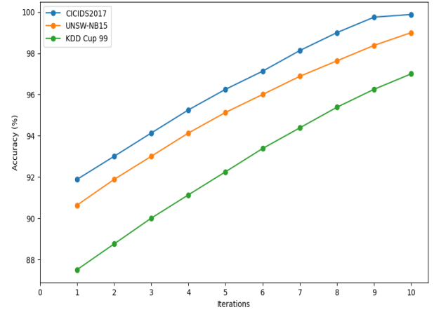
Fig. 2: Accuracy for FL under different iterations and 10 nodes
