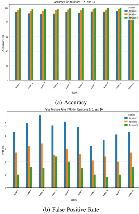
Fig. 3: Performance evaluation under heterogeneous data sets
