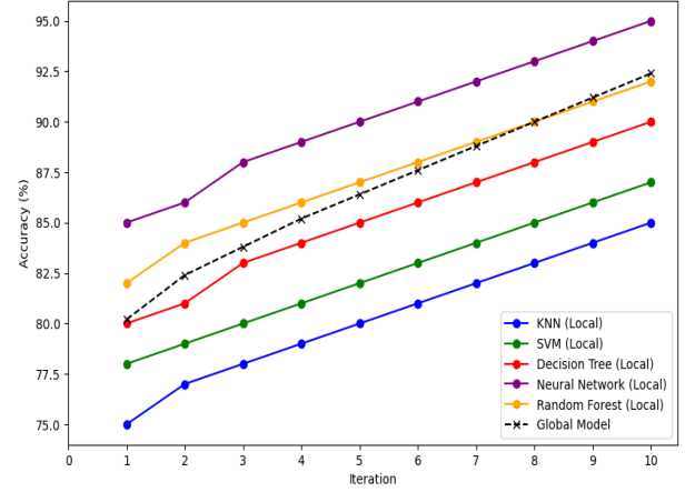
Fig. 4: Accuracy of FL systems under different Machine learning Models at Client Side.
