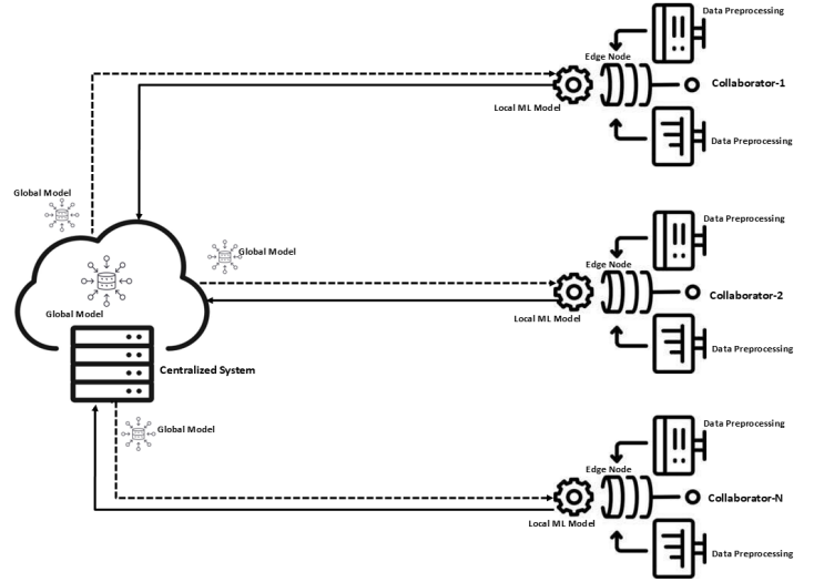
Fig. 1: FL System Architecture with Edge Nodes
