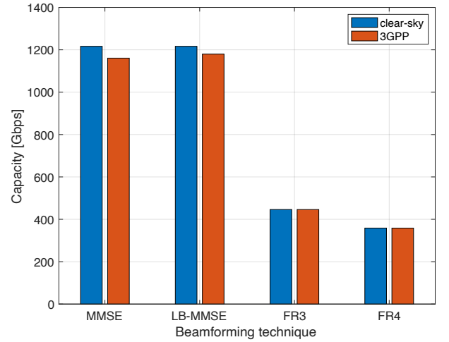
(b) System capacity with user-centric beamforming.
