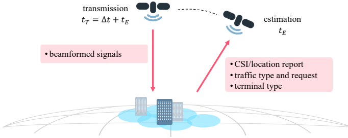
(a) System model for user-centric beamforming.
