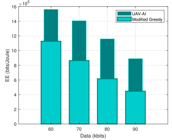
(b) EE versus the transmitted data size for a fixed number of UEs.
