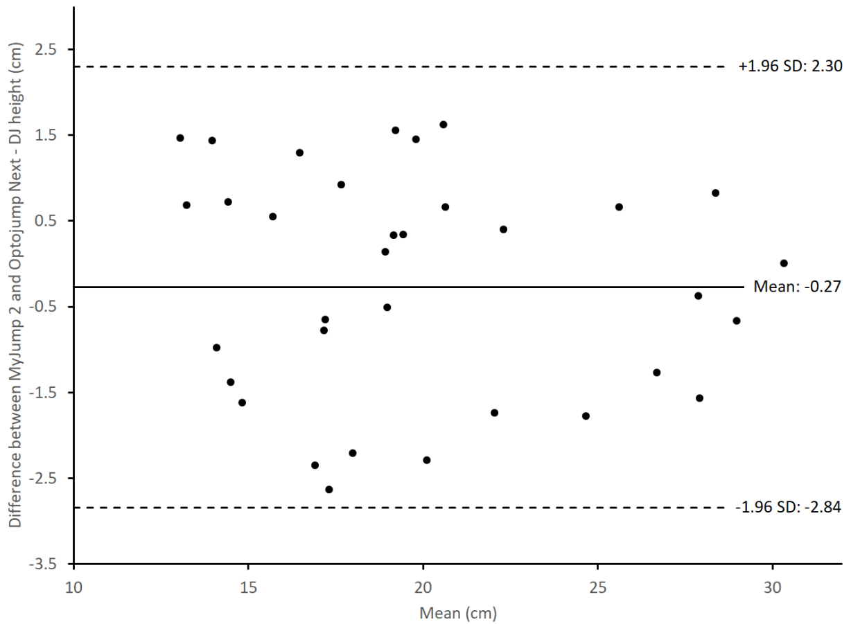
Fig 4.3 Bland-Altman limits of agreement between the MyJump 2 app and Optojump Next for drop jump (DJ) height (cm) with 95% (+1.96) upper and 95% lower (-1.96) limits (dotted lines) and mean difference (solid line).
