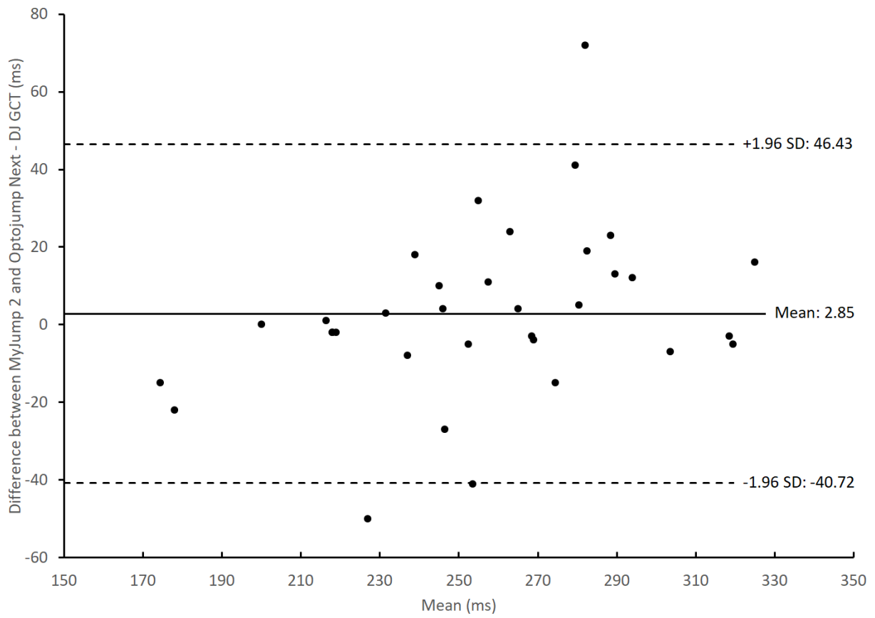
Fig 4.4 Bland-Altman limits of agreement between the MyJump 2 app and Optojump Next for drop jump (DJ) ground contact time (GCT) (ms) with 95% (+1.96) upper and 95% lower (-1.96) limits (dotted lines) and mean difference (solid line).
