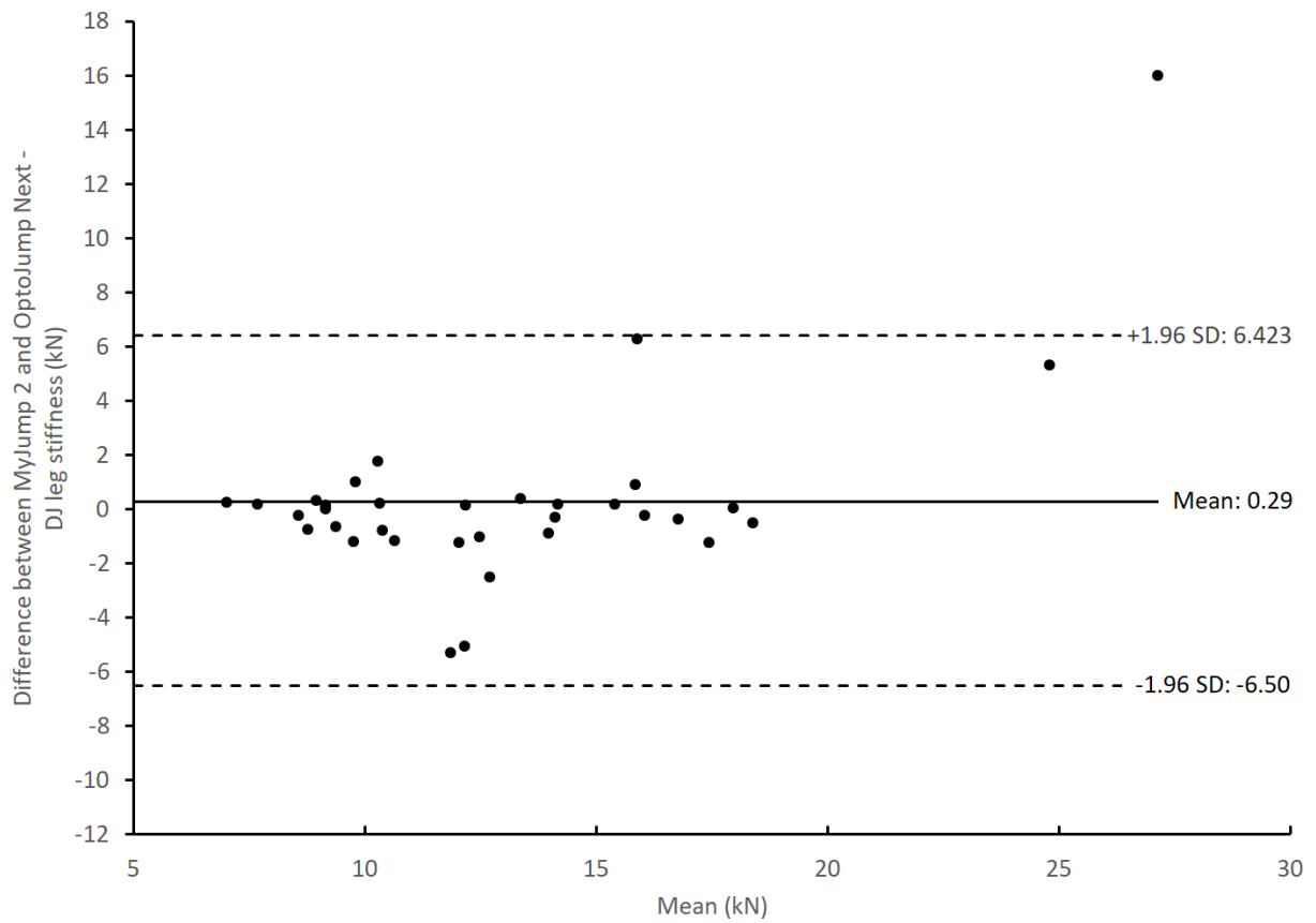
Fig 4.7 Bland-Altman limits of agreement between the MyJump 2 app and OptoJump Next for leg stiffness (kN) with 95% (+1.96) upper and 95% lower (-1.96) limits (dotted lines) and mean difference (solid line).
