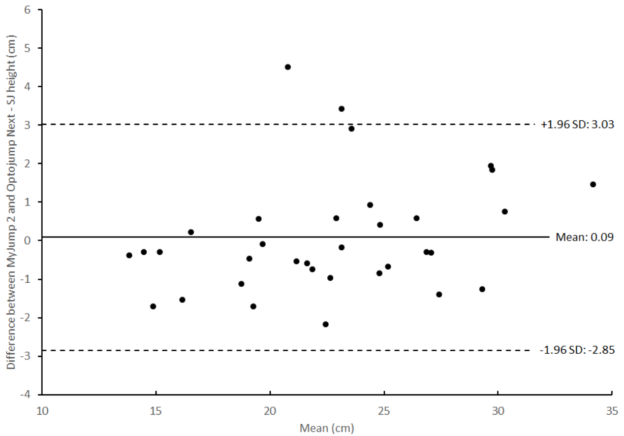
Fig 4.1 Bland-Altman limits of agreement between the MyJump 2 app and Optojump Next for Squat jump (SJ) height (cm) with 95% (+1.96) upper and 95% lower (-1.96) limits (dotted lines) and mean difference (solid line).
