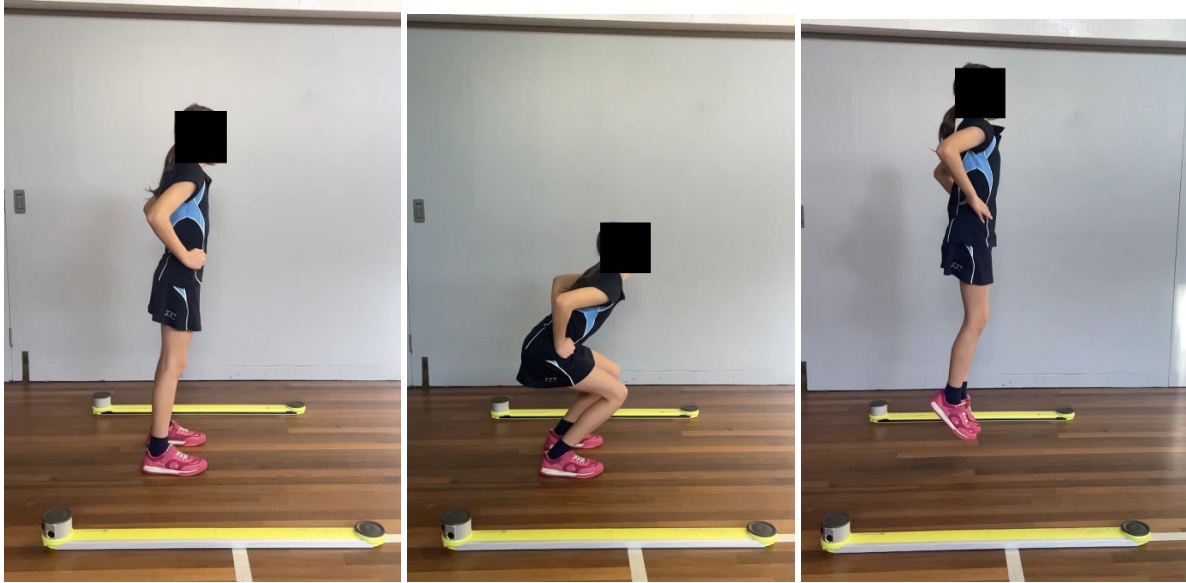
Fig 3.2 Illustration of the participant's starting position and location of the Optojump Next system during a countermovement jump (CMJ).
