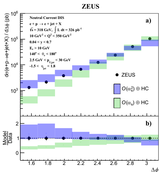
Fig. 5 a The differential cross section d\sigma(e + p \rightarrow e + \text{jet}^{\text{lead}} + X)/d\Delta\phi as a function of the azimuthal correlation angle \Delta\phi in the full fiducial region. The vertical error bars represent the statistical and systematic uncertainties added in quadrature. The green and blue bands represent the perturbative QCD calculations at \mathcal{O}(\alpha_s) and \mathcal{O}(\alpha_s^2) accuracy, respectively, corrected for hadronisation effects (HC). b Ratio of model/data
