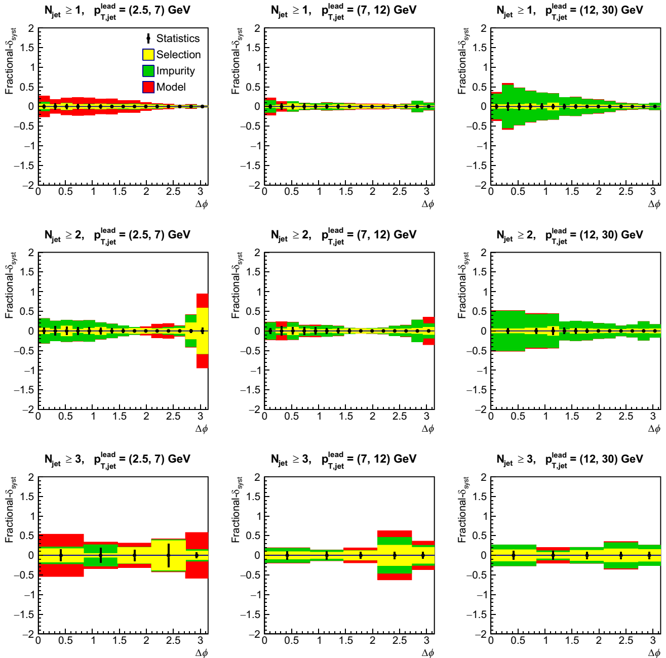
Fig. 15 Breakdown of the systematic uncertainty in various ranges of N_{jet} and p_{T,jet} compared to the statistical uncertainty. Other details are as in the caption to Fig. 4
