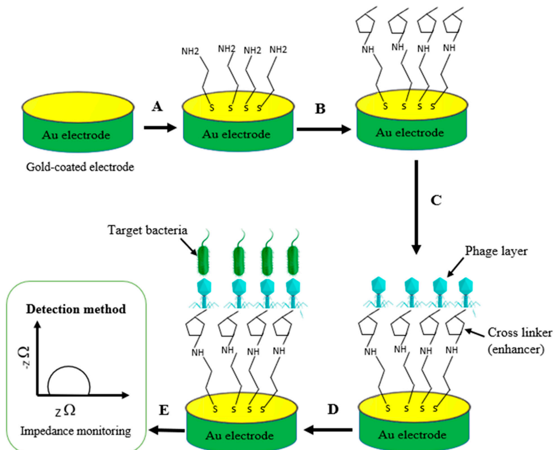
Figure 5. Schematic illustration of phage-based impedimetric biosensor, showing steps involved in phage immobilization and target bacteria detection: (A) surface modification of gold electrode using chemical linker (e.g., cysteamine); (B) cross-linker/enhancement using 1,4 dithiocyanate (PDICT); (C) immobilization of phages and treatment with ethanolamine to block nonspecific binding; (D) capture of target bacteria; and (E) impedance measurement (detection of target pathogen).
