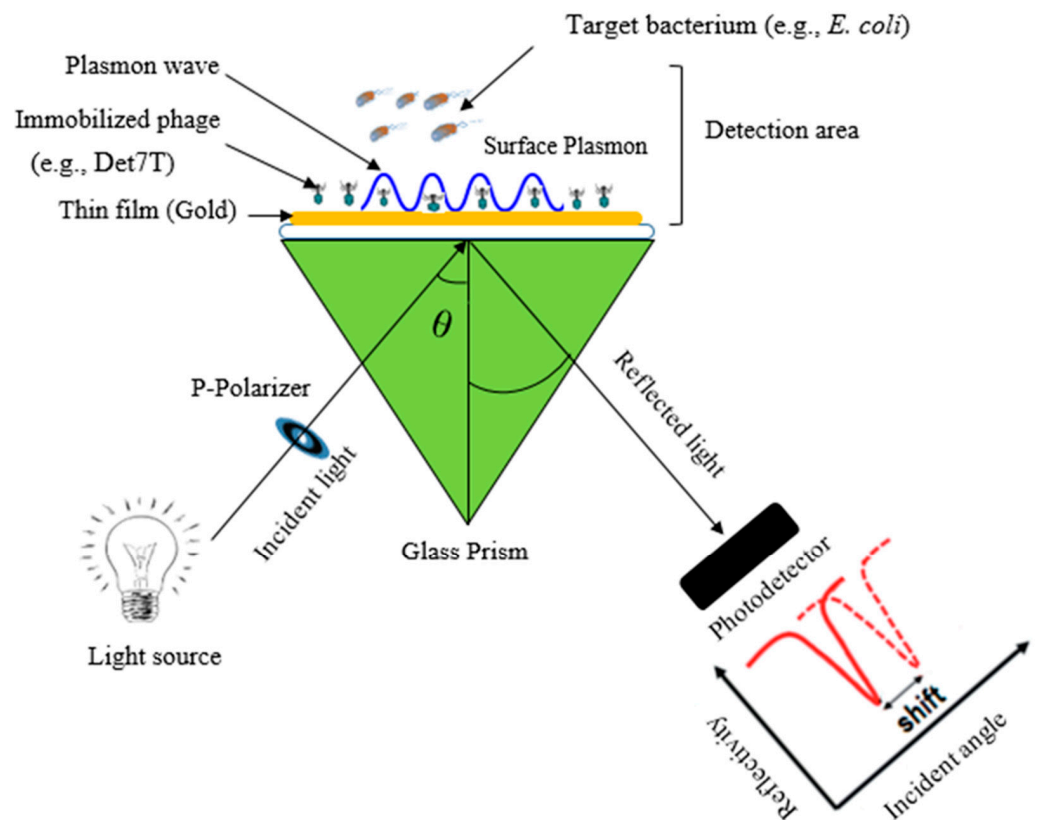
Figure 4. Schematic diagram illustrating the working principle of a surface plasmon resonance sensor (SPR) using bacteriophages.
