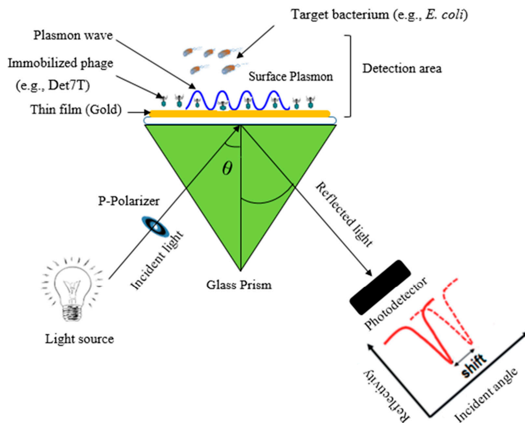
Figure 4. Schematic diagram illustrating the working principle of a surface plasmon resonance sensor (SPR) using bacteriophages.
