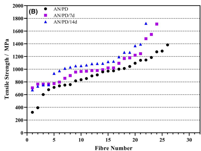
FIGURE 8 Individual filament strength values for fibers that were annealed (AN—left) with respect to fibers that were annealed, washed with HCl for 10 min and coated with polydopamine (AN/PD—right). Comparison of results for up to 14 d degradation in water at 37^{\circ}\text{C} . Values for each data set are plotted in ascending order to facilitate comparisons and to identify any outliers
