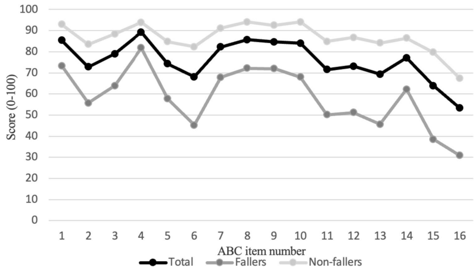
Fig. 1 Mean scores of each item on the ABC-16 scale
