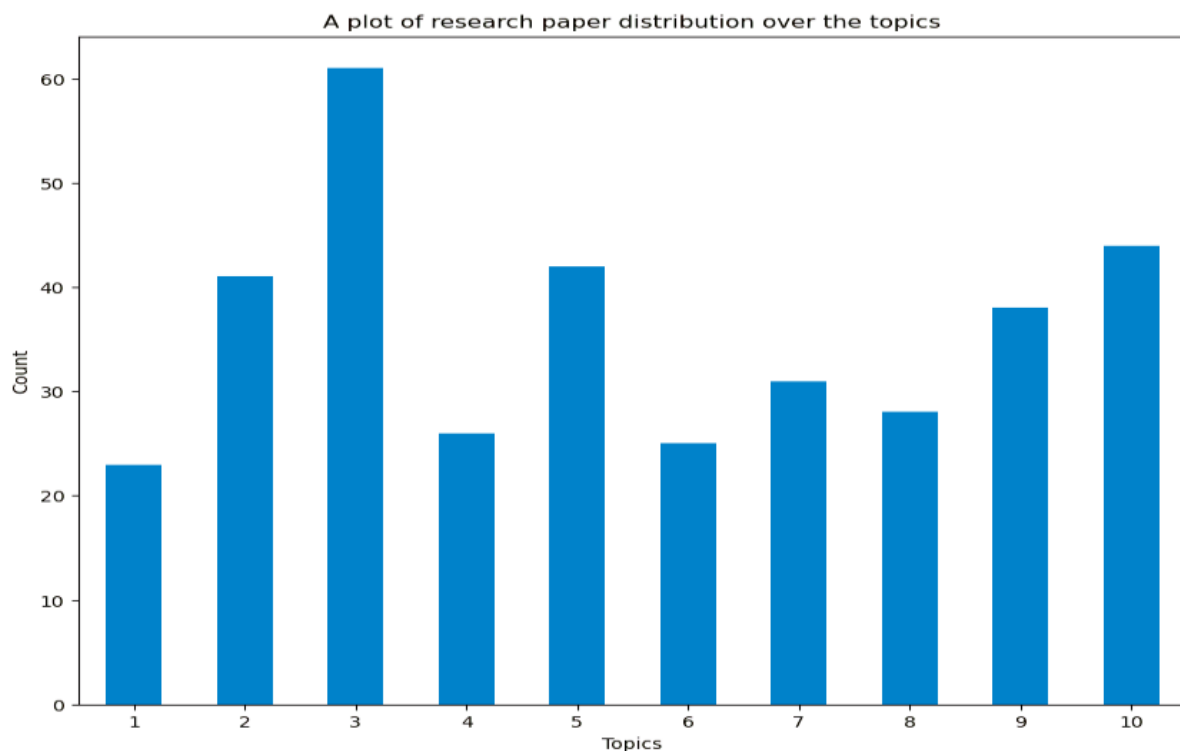
Figure 10. Topic distribution.
