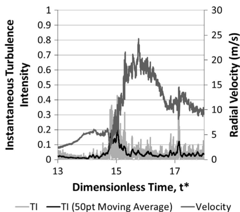
Fig. 8. Turbulence intensity during a single run at z/D=0.02 .
