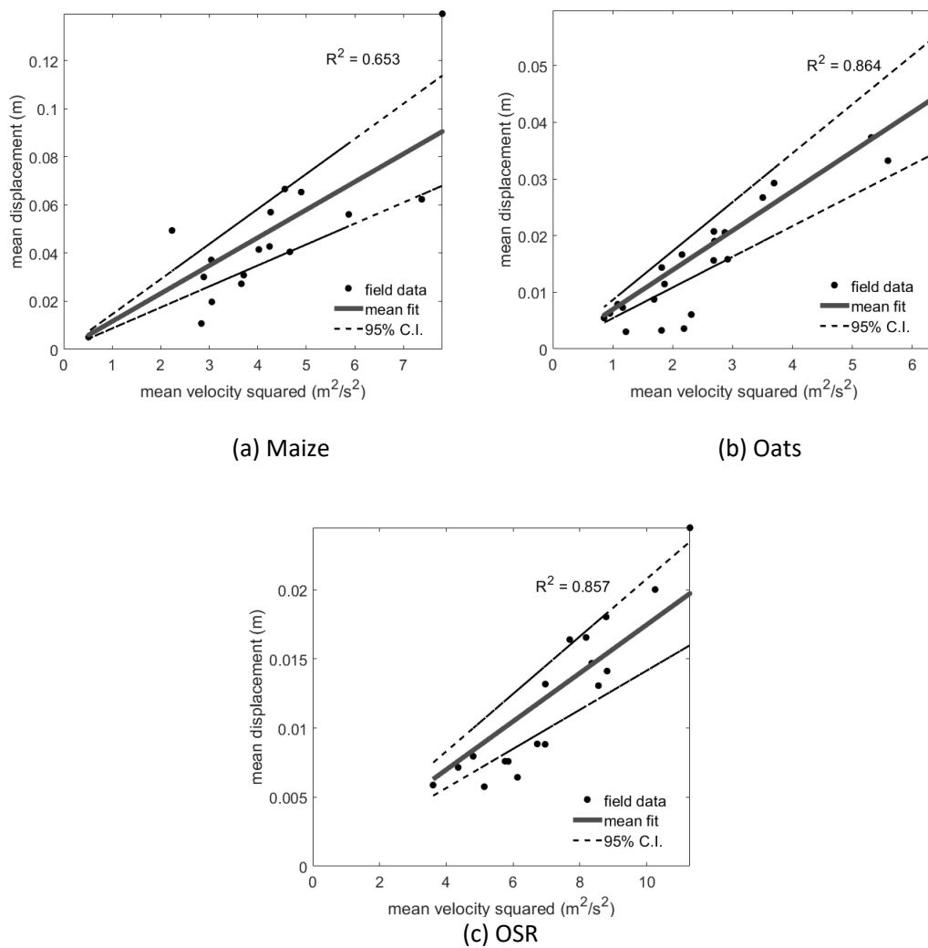
Figure 9 Mean displacement of all datasets plotted against mean velocity squared.
