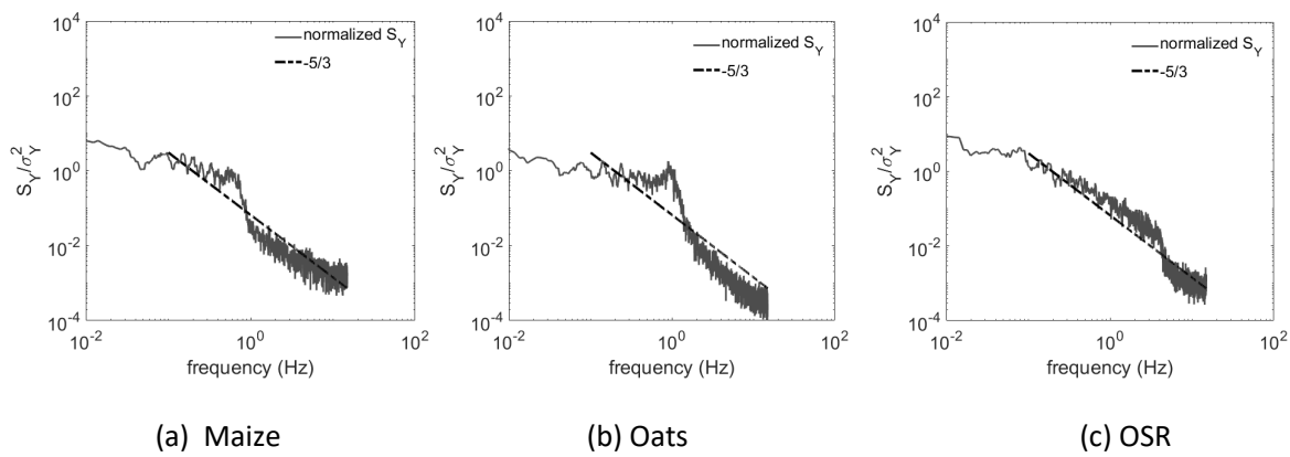
Figure 7 Typical streamwise displacement spectra
