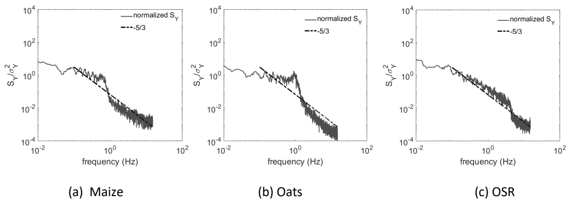
9 10 11 12 13 Figure 7 Typical streamwise displacement spectra
