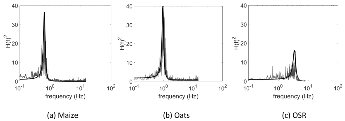
Figure 8 Mechanical admittance functions
