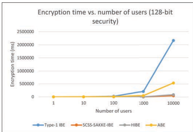
Figure 11: Encryption time vs. number of users in 128-bit security level 940
