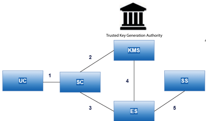
Figure 4: Main components of SCSS-SAKKE-IBE
