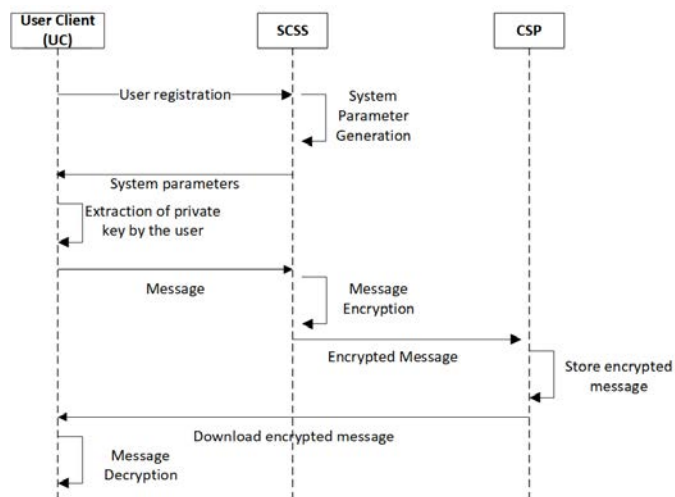
Figure 5: Main secure cloud storage scenario
