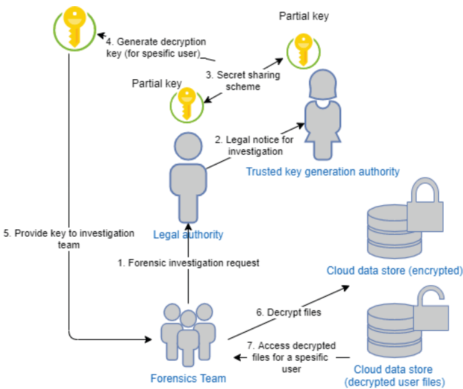
Figure 6: Digital forensic investigation on encrypted data on the cloud
