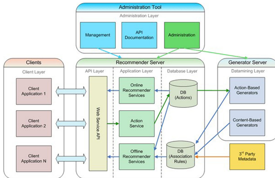
Fig. 3. Web application architecture
