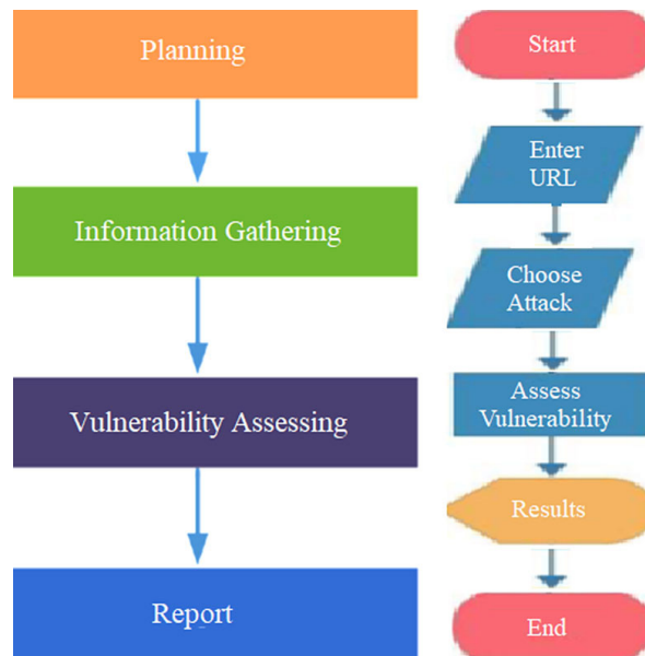
Fig. 8. Security assessment model of web application
