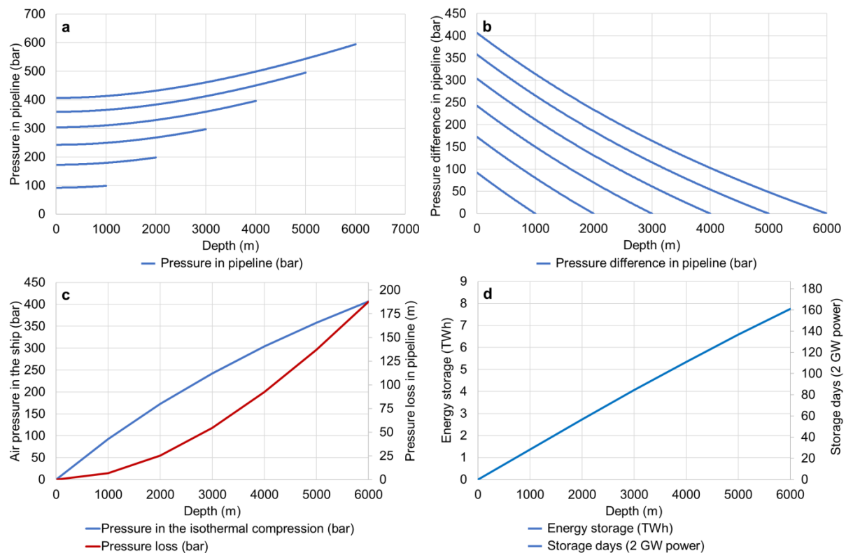
Figure 7. IDO-CAES energy storage estimation, showing (a) the pressure of the compressed air in the vertical pipeline, (b) the pressure difference between the compressed air pipeline and the ocean, (c) the compressed air pressure in the ship and head loss, and (d) the energy storage capacity of the system in the deep ocean.
