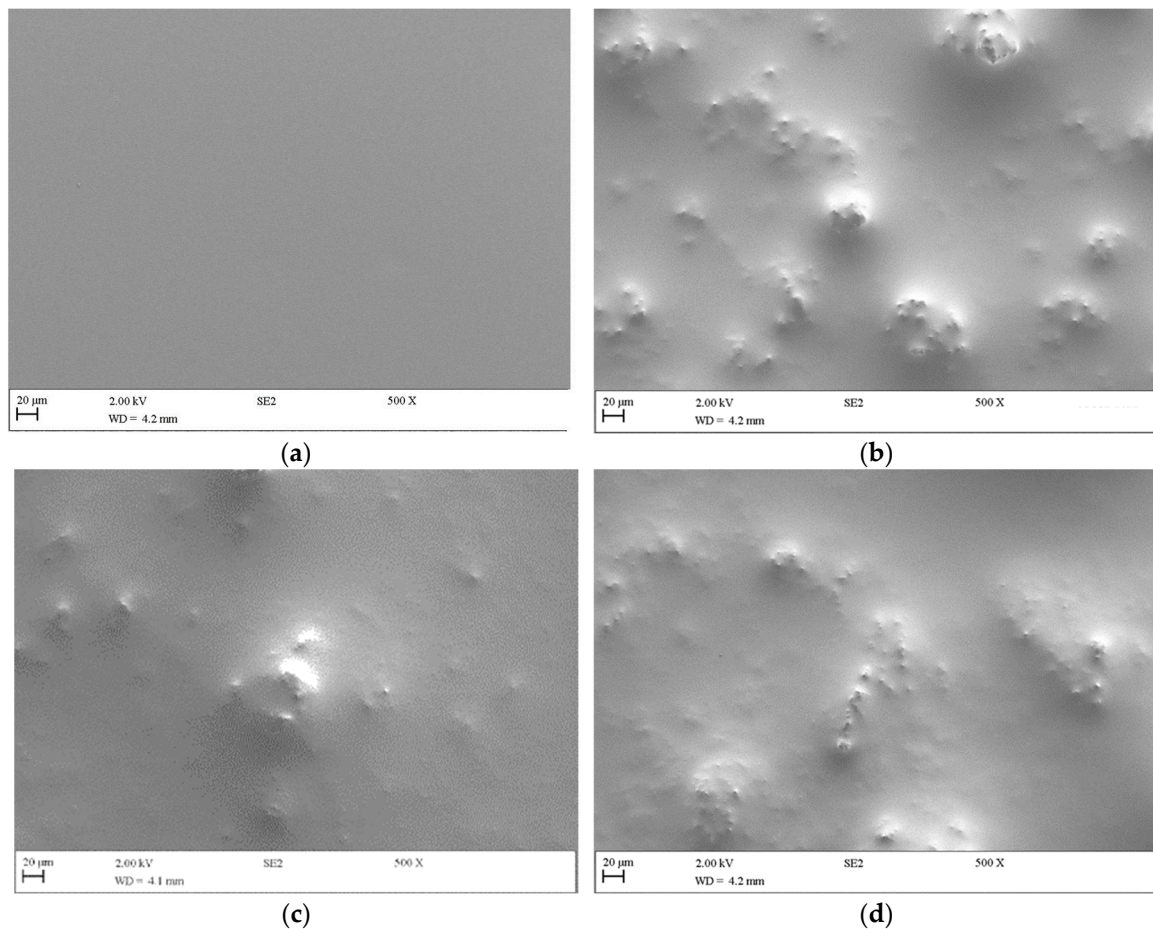
Figure 4. SEM images of (a) PDMS, (b) p-MWCNT/PDMS, (c) f-MWCNT_N/PDMS, and (d) f-MWCNT_N600/PDMS composites (magnification of 500×).
