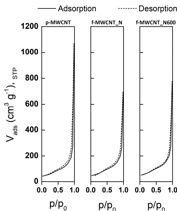
Figure 1. N 2 adsorption–desorption isotherms at −196 °C for pristine multi-walled carbon nanotubes (p-MWCNT), nitric acid-functionalized multi-walled carbon nanotubes (f-MWCNT_N), and f-MWCNT_N heated at 600 °C (f-MWCNT_N600).
