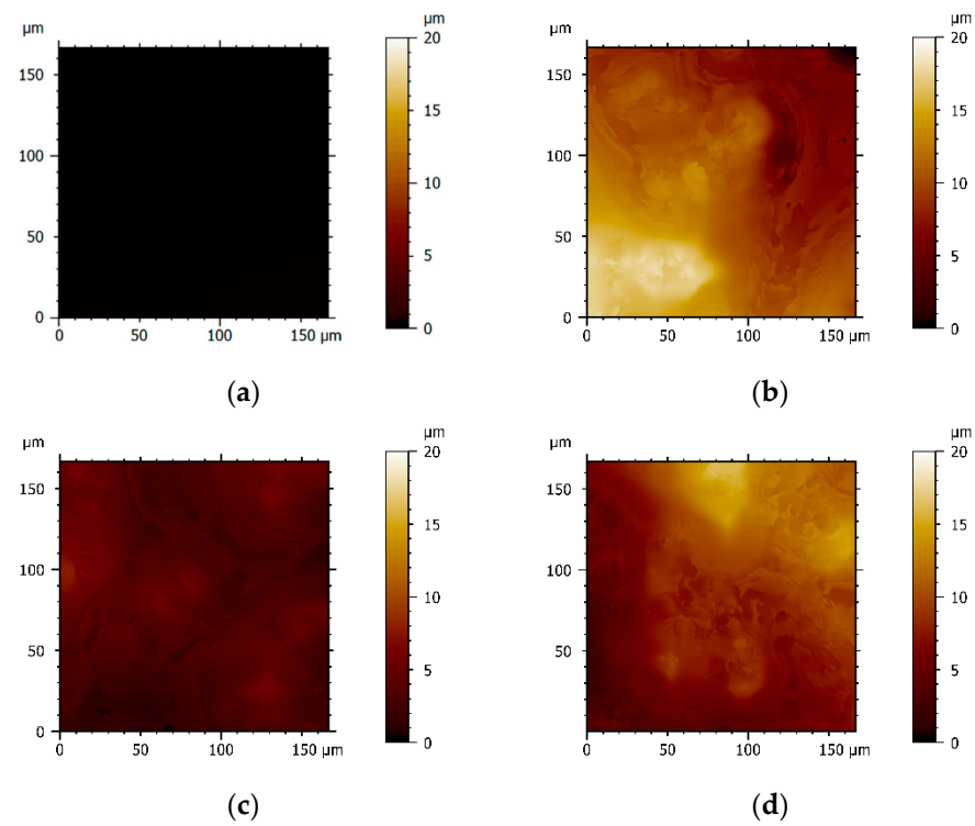
Figure 2. Representative 2D profilometry images of (a) PDMS, (b) p-MWCNT/PDMS, (c) f-MWCNT_N/PDMS, and (d) f-MWCNT_N600/PDMS (scan area of 170 \times 170 \mu\text{m} ). The vertical color bars represent the range of surface heights ( z -range) of the images.
