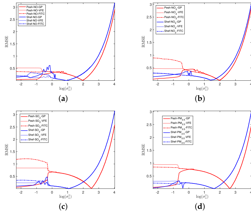
Figure 5. Relationship of \sigma_n^2 with four pollutants prediction RMSE: (a) NO, (b) NO 2 , (c) SO 2 , (d) PM 2.5 .
