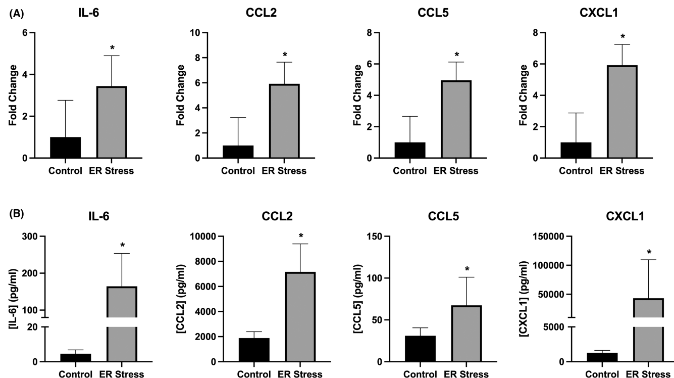
FIGURE 4 Gene expression (A) and released protein levels (B) of IL-6, CXCL1, CCL2 and CCL5 from C2C12 myotubes treated with 0.1 g/ml of the ER stress-inducing compound tunicamycin for 24h. Data are presented as mean ± SEM ( n = 3-6 ), * p \leq 0.05 .
