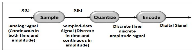
Fig. 1: Sampling, quantizing, and encoding.
