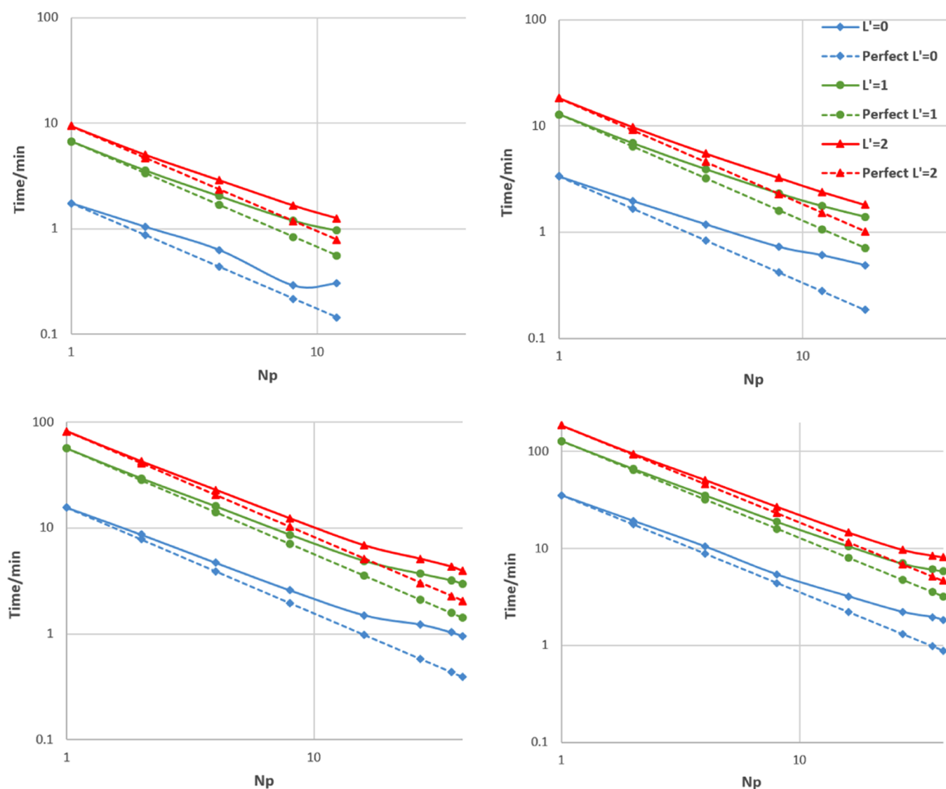
Figure 10. Strong scaling, both actual and perfect, on log–log axes for all four water boxes: (top left) 5184 atoms in a (38 Å) 3 box; (top right) 10125 atoms in a (47 Å) 3 box; (bottom left) 46875 atoms in a (78 Å) 3 box; and (bottom right) 107811 atoms in a (103.5 Å) 3 box.
