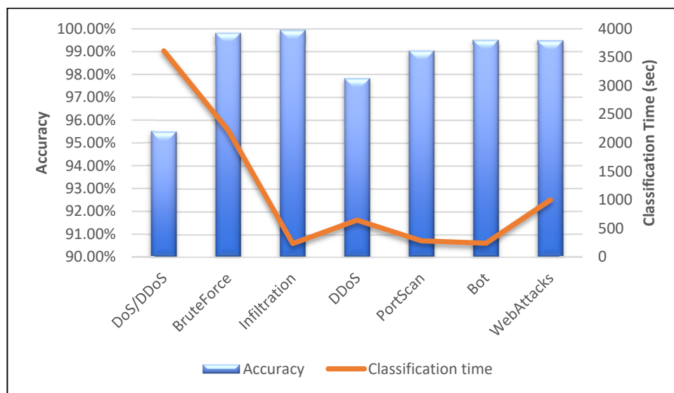
Figure 14. Accuracy vs. classification time.
