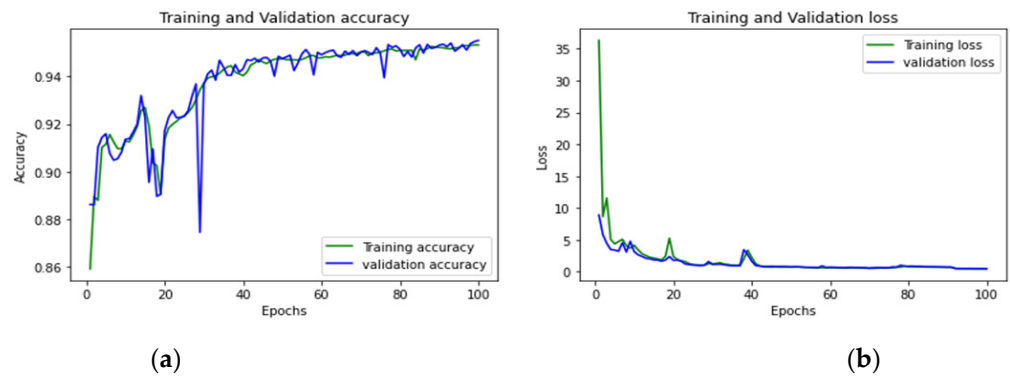
Figure 16. (a,b): Wednesday: Accuracy curve and Loss curve.
