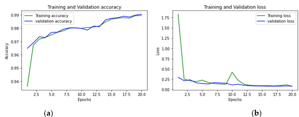
Figure 21. (a,b): Friday afternoon PortScan: Accuracy curve and Loss curve.
