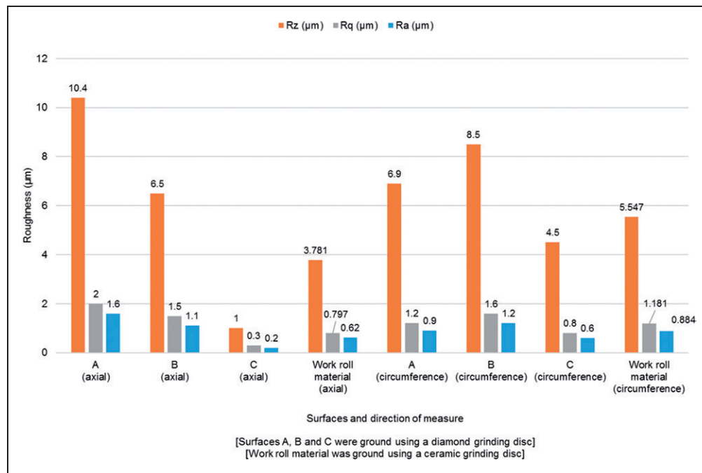
Figure 12. Roughness measurements.
