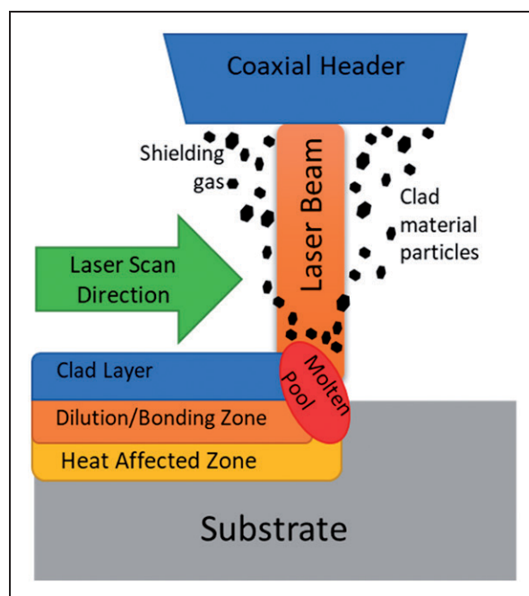
Figure 3. Laser cladding blown powder method.
