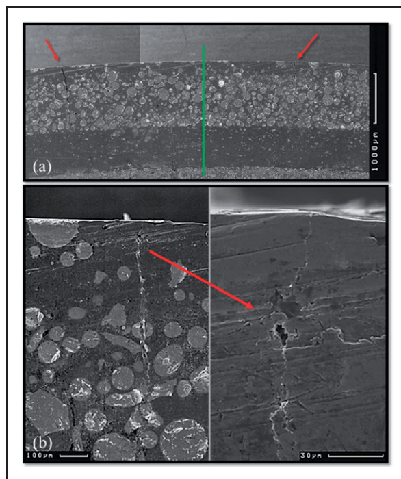
Figure 24. (a) Bending axis plane (green line) and cracks at either end (red arrows) for SEM clad test specimen; (b) Possible microstructure flaw or porosity that may have contributed to cracking.
