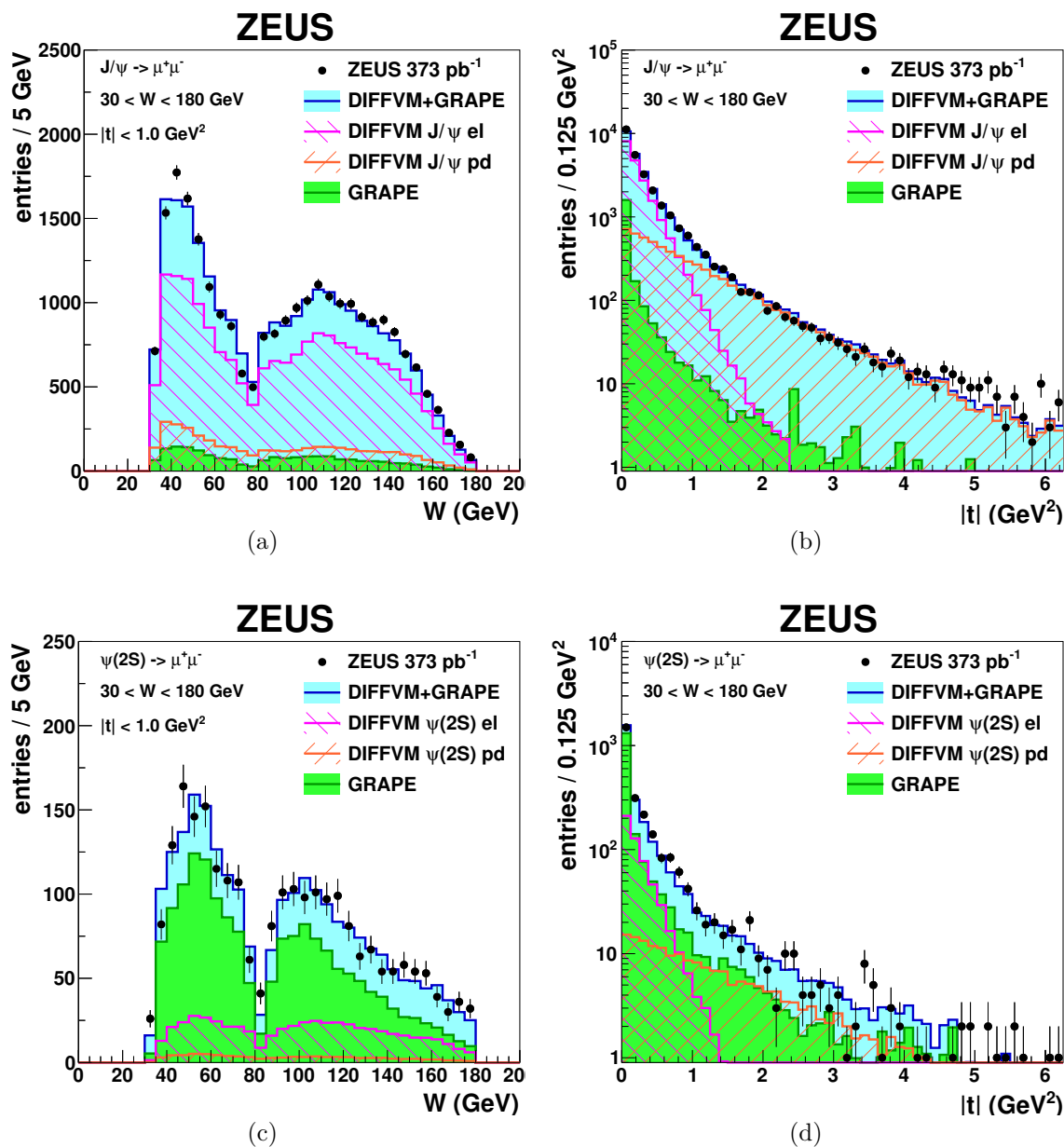
Figure 5. Distributions of (a, c) W and (b, d) |t| reconstructed for the decay of (a, b) J/\psi(1S) and (c, d) \psi(2S) mesons to a \mu^+\mu^- pair in photoproduction events (solid circles), with error bars denoting statistical uncertainties. DIFFVM MC distributions for simulated events are shown for elastic (magenta hatched histogram) and proton-dissociative (orange hatched histogram) processes separately. The total sum of all contributions (blue solid histogram) as well as the GRAPE MC contribution from Bethe-Heitler processes (green solid histogram) is also shown. The statistical uncertainties on the MC histograms are not shown; they are about 40% of the size of the statistical uncertainties in the data.
