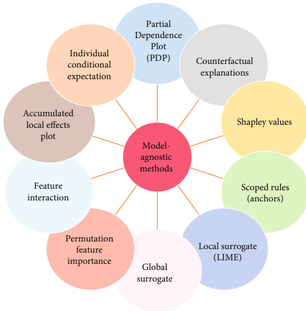
FIGURE 6: Model-agnostic methods.
