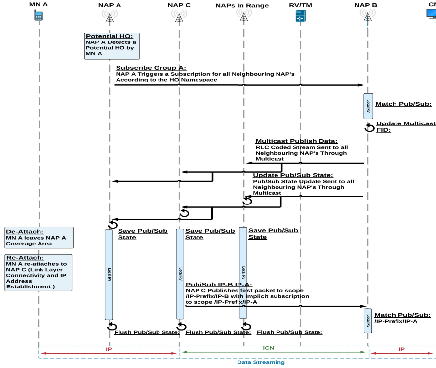
Fig. 3: Handover Sequence Diagram.
