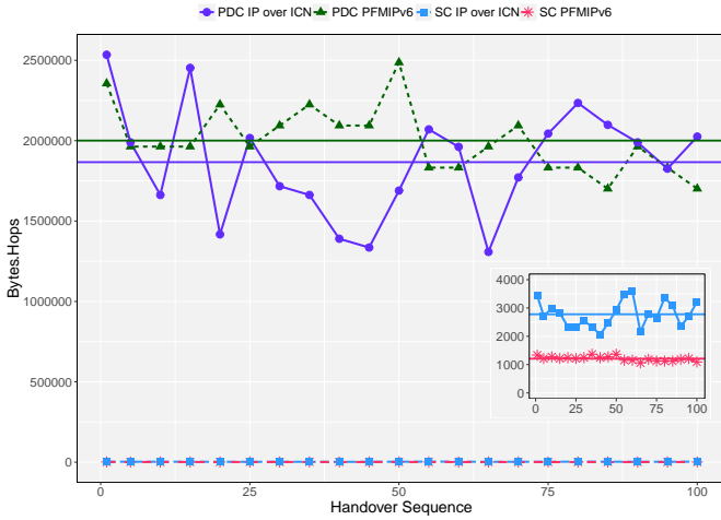
Fig. 7: Averaged Packet Delivery Cost (PDC) and Signalling Cost (SC) for PFMIIPv6 vs. IP over ICN with respect to 100 sequent Handover's.
