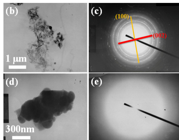
Figure 4. (a) X-ray diffraction spectra of graphene/PET and ZnO (40, 75, and 160 nm thickness)/graphene/PET; (b,c) TEM image and SAED pattern of graphene/PET; (d,e) TEM image and SAED pattern of ZnO/graphene/PET.
