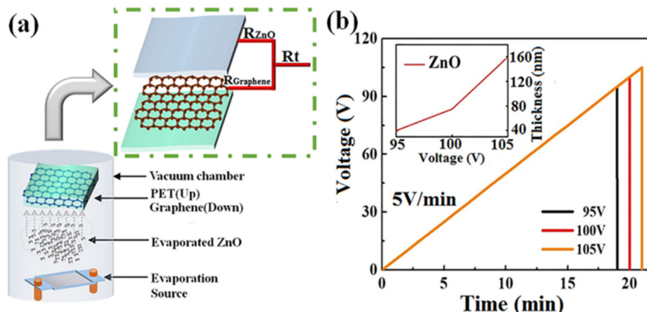
Figure 1. Experimental method and technology: (a) vacuum evaporation plating method and a schematic diagram of the parallel resistance of amorphous ZnO/graphene/PET film; (b) technological parameter graph of the ZnO deposition process.
