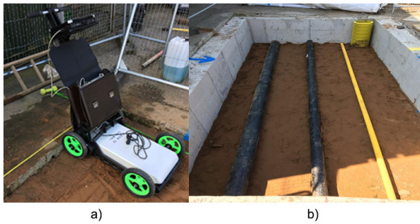
FIGURE 7. a) is the modular, off the shelf terrestrial based system (ZOND 12), b) is the on-site experimental environment.
