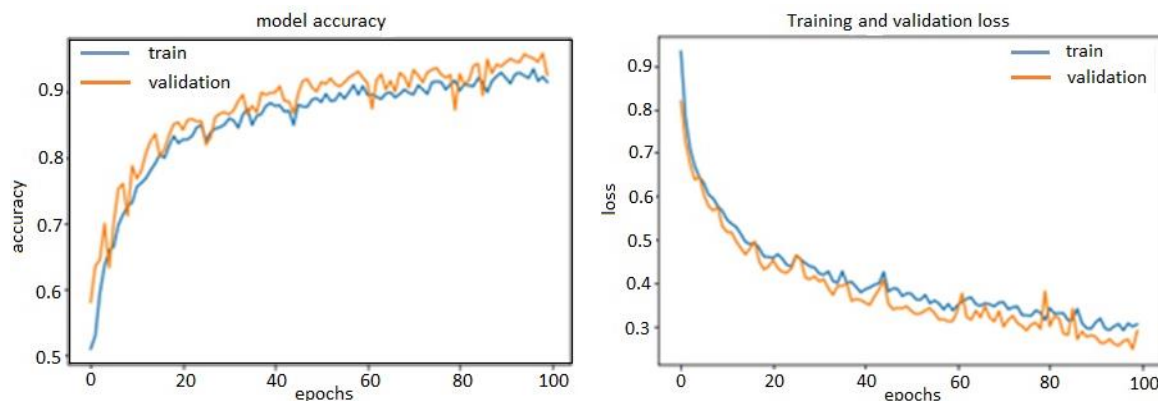
Figure 13. Accuracy and loss model of FFT_1D-CNN.
