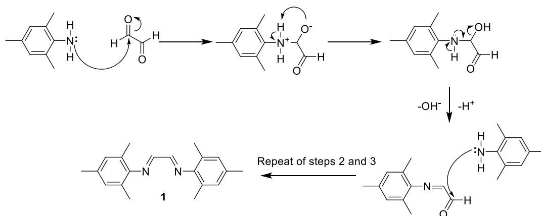
Figure 27. Reaction scheme for the synthesis of N,N' -bis(2,4,6-trimethylphenyl)ethanediamine ( 1 ).
