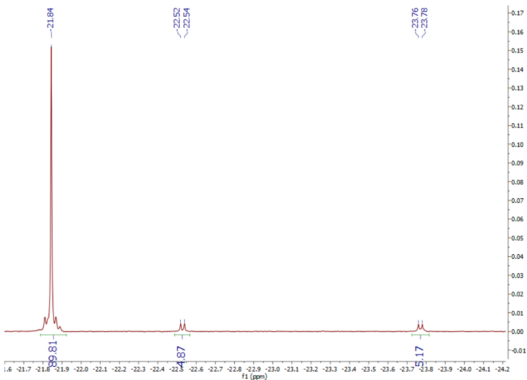
Figure 66. Hydride region demonstrating the major and minor species in solution following addition of three equivalents ethylenediamine to [\text{Ir}(\text{IMes})(\text{pyridine})_3(\text{H})_2] .
