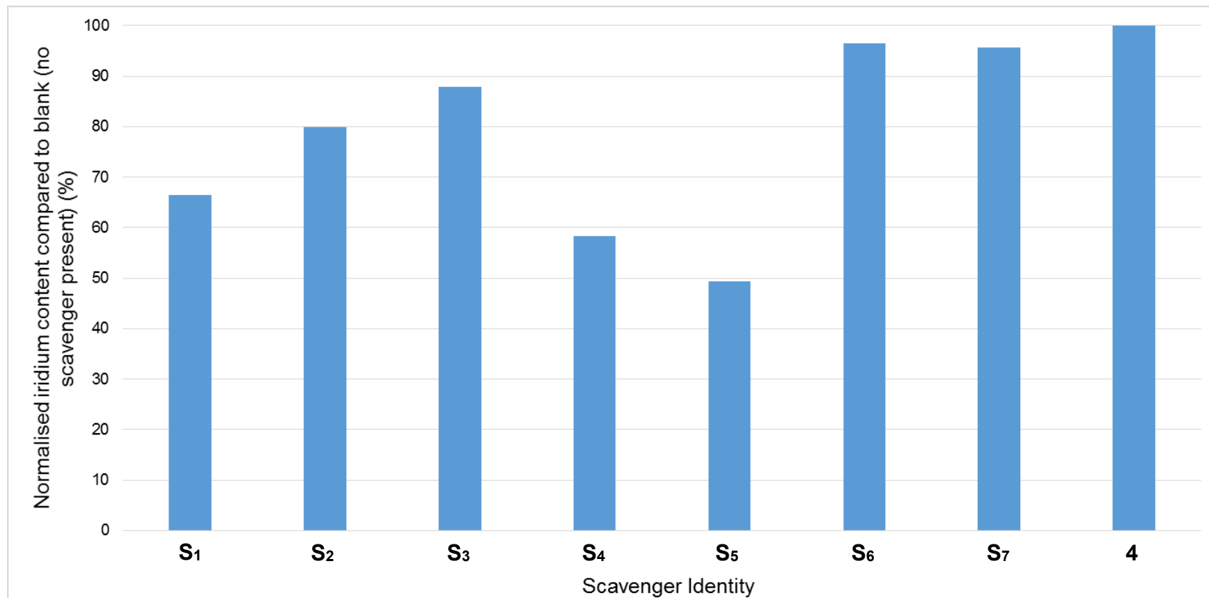
Figure 73. Iridium present in samples following the addition of 10 mg of scavengers S1-S7 and with no scavenger added ( 4 ) after 12 days normalised to iridium content of the blank sample with no scavenger added.
