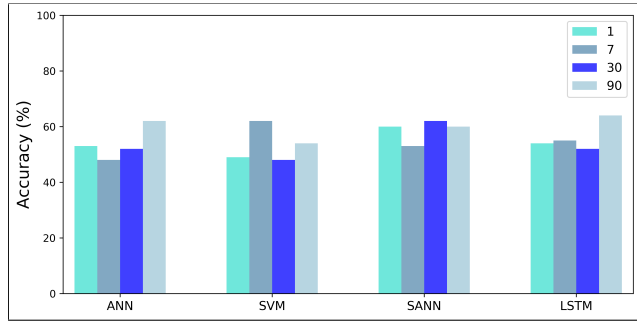
Fig. 10: Accuracy of the classification models for n th day forecast in Interval III.
