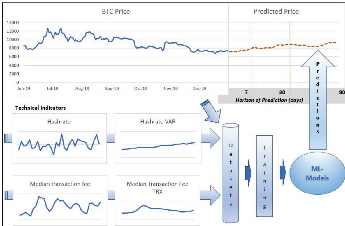
Fig. 2: ML-based timeseries forecast using technical indicators
