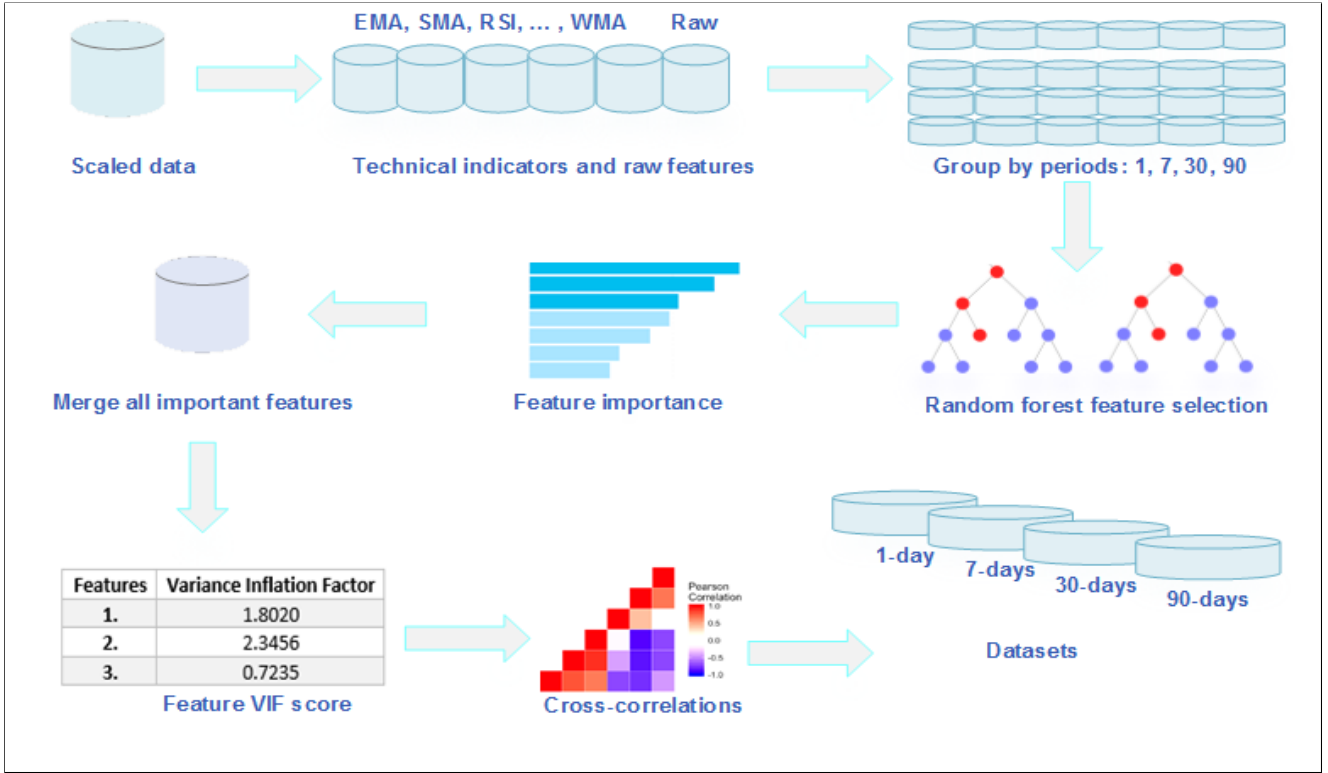
Fig. 5: Feature selection process
