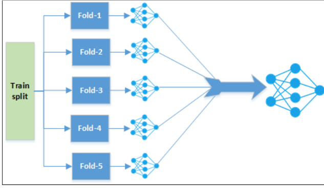
Fig. 6: Architecture of the densely connected SANN wherein separate ANN are trained on unique folds of the trained split. The outputs from the trained sub-models are used as the input for the final model, which uses the best input for making its own forecasts.
