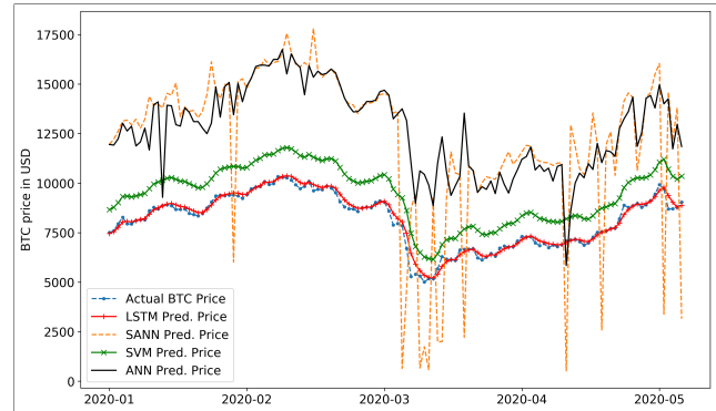
Fig. 9: The trained models based on Interval III are used to forecast the BTC prices for data after December 2019 – which is excluded from the train and test sets. It shows LSTM performs the best, followed by SVM. ANN and SANN have similar patterns, although SANN has more fluctuations.
