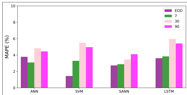
Fig. 7: MAPE of the regression models for n^{\text{th}} days forecasts in Interval III.
