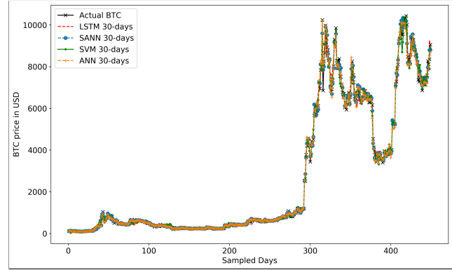
Fig. 8: Based on the 30-days regression models and a sampled dataset (shifted by 30 days) from the entire study period is shown. It shows all the models are quite close to each other and follow the BTC prices closely.
