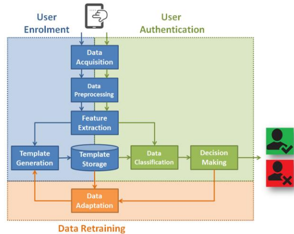
Fig. 3. A touch dynamics authentication framework
