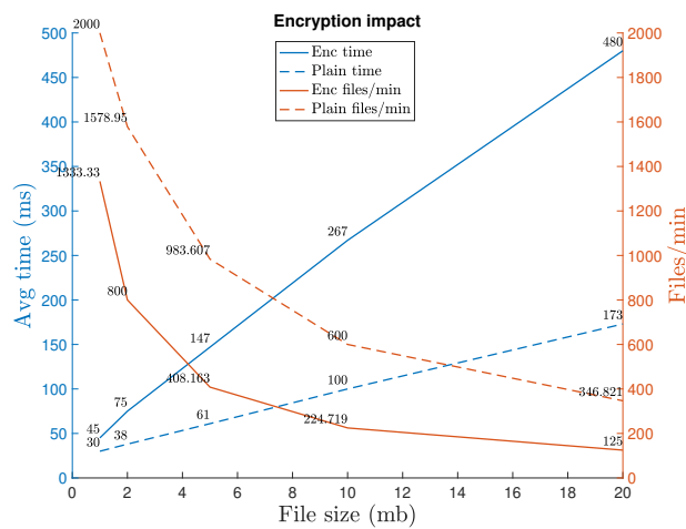
Fig. 6: Cydon’s Cryptographic Overhead for different file sizes
