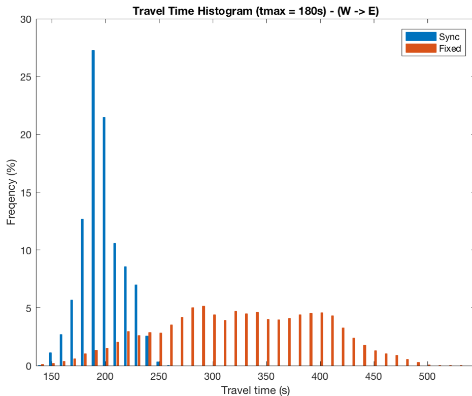
Figure 12. Travel time distribution: fixed time Traffic Light Control System (TLCS) vs. synchronized Adaptive Traffic Light Control System (ATLCS).
