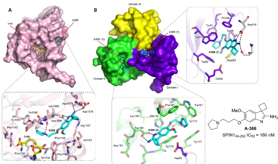
Figure 1. Crystal structure of A-366 with G9a and SPIN1. (A) Structural of A-366 (cyan) in complex with G9a (pink) (PDB ID 4NVQ). 24 (B) Structure of A-366 (cyan) in complex with SPIN1 (PDB ID 6I8Y).
