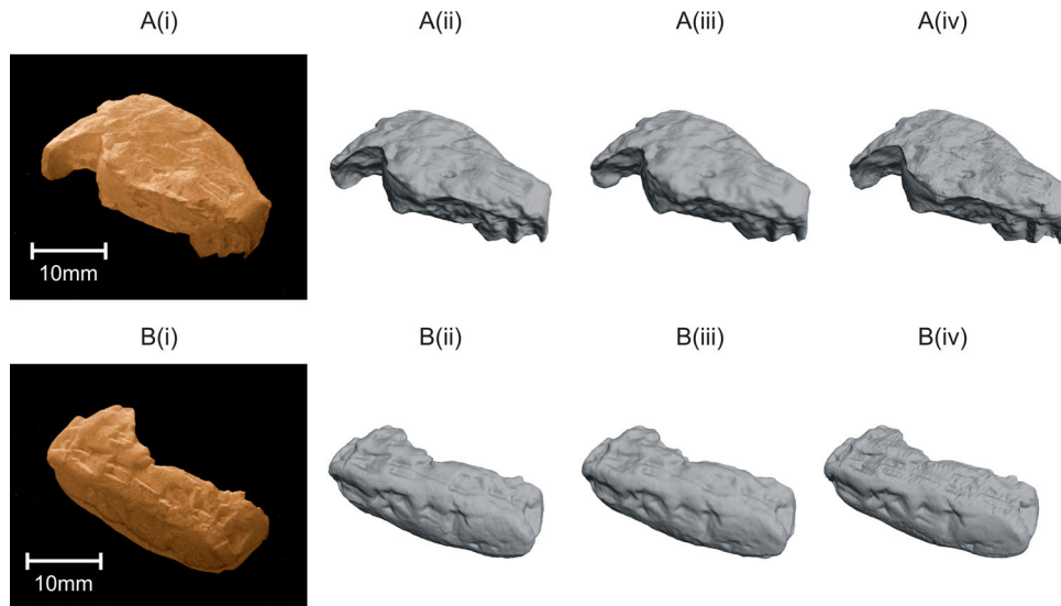
Figure 11. (Ai) and (Bi) are photographs of the two 3D printed cuneiform tablet fragment facsimiles (created from scans of W 18349 and Wy 777) used to test the acquisition precision. (Aii) and (Bii) are 3D models created using the rotary acquisition system with the DSLR camera. (Aiii) and (Biii) are 3D models created using the rotary acquisition system with the smartphone system. (Aiv) and (Biv) are 3D models created using the DAVID-SLS-2 structured light scanner.
