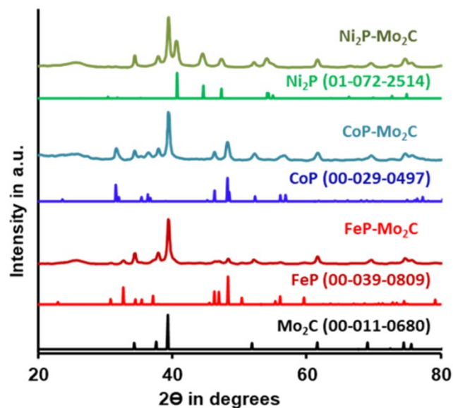
Figure 1. PXRD patterns of metal phosphide (MP) deposited carbide composites (MP- \text{Mo}_2\text{C} ) and the corresponding reference patterns with the PDF numbers.
