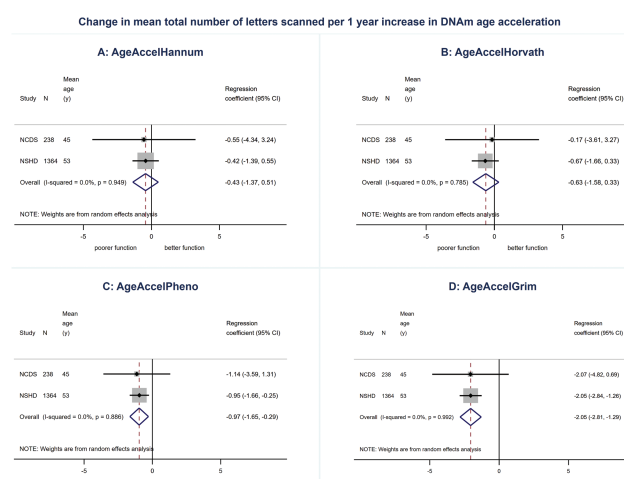
Figure 5. Association between (A) AgeAccelHannum, (B) AgeAccelHorvath, (C) AgeAccelPheno, (D) AgeAccelGrim and total number of letters scanned adjusted for sex and age.
