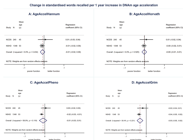
Figure 4. Association between (A) AgeAccelHannum, (B) AgeAccelHorvath, (C) AgeAccelPheno, (D) AgeAccelGrim and standardized total number of words recalled adjusted for sex and age.
