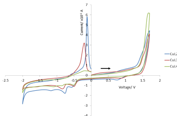
Figure 7. Cyclic voltammograms of [\text{CuL}^2]^{2+} , [\text{CuL}^3]^{2+} and [\text{CuL}^4]^{2+} at 0.2 V/s. Data collected in acetonitrile with tetrabutylammonium perchlorate as a supporting electrolyte at RT using a Ag/AgCl reference electrode.
