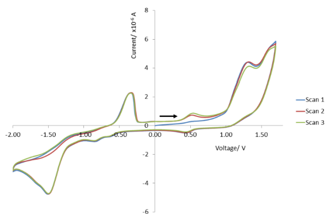
Figure 8. Consecutive cyclic voltammograms of [\text{CuL}^1]^+ at 0.2 V/s. Data collected in acetonitrile with tetrabutylammonium perchlorate as a supporting electrolyte at RT using a Ag/AgCl reference electrode.
