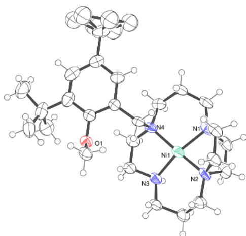
Figure 6. ORTEP representation (50% thermal ellipsoids) of the X-ray crystal structure of [NiL 2 ] 2+ with all non-H atoms labelled. Water molecules and perchlorate anions have been removed for clarity
