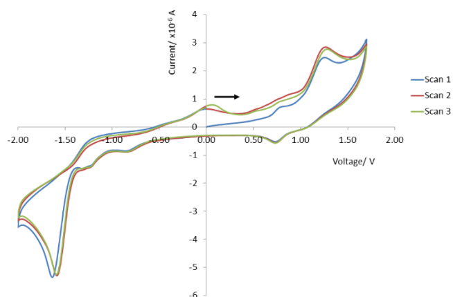
Figure 10. Consecutive cyclic voltammograms of [\text{NiL}_1]^+ 0.2 V/s. Data collected in acetonitrile with tetra-butyl ammonium perchlorate as a supporting electrolyte at RT using a Ag/AgCl reference electrode.
