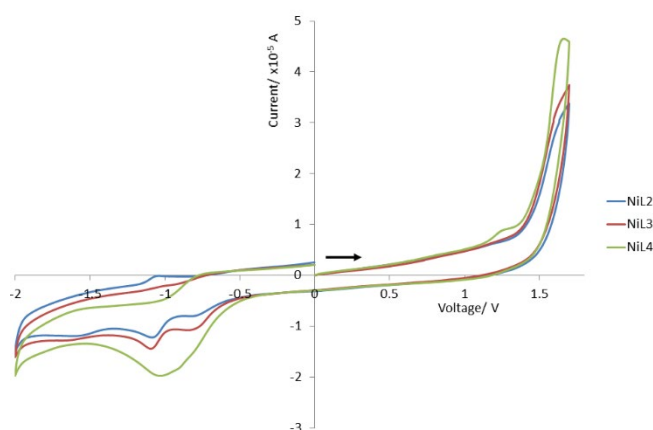
Figure 9. Cyclic voltammograms of [\text{NiL}^2]^{2+} , [\text{NiL}^3]^{2+} and [\text{NiL}^4]^{2+} recorded at 0.2 V/s. Data collected in acetonitrile with tetrabutylammonium perchlorate as a supporting electrolyte at RT using a Ag/AgCl reference electrode.
