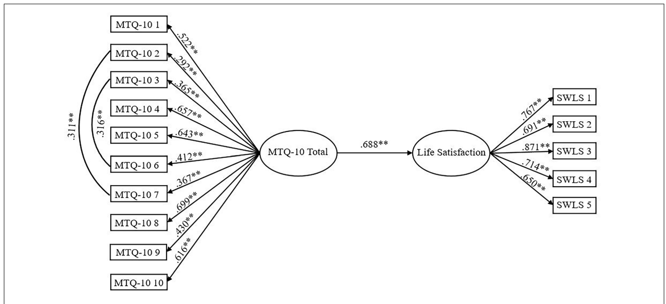
FIGURE 3 | MTQ-10 as a predictor of life satisfaction. Ellipses represent latent variables; measured variables are represented by rectangles; error is not shown but was specified for all variables. ** p < 0.001 (using bootstrap significance estimates).
