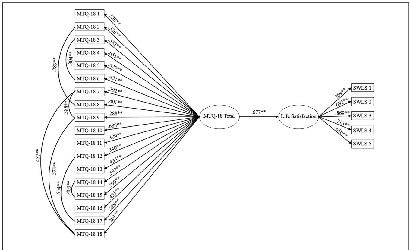
FIGURE 2 | MTQ-18 as a predictor of life satisfaction. Ellipses represent latent variables; measured variables are represented by rectangles; error is not shown but was specified for all variables. ** p < 0.001 (using bootstrap significance estimates).
