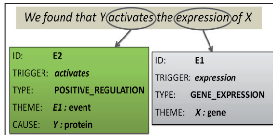
Figure 1. Bio-Event Representation
