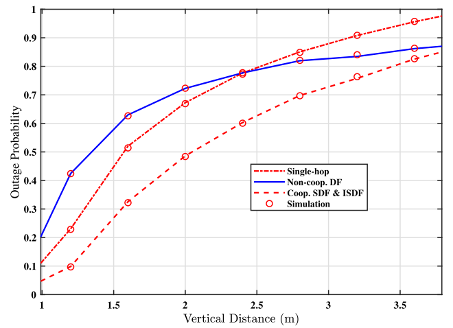
Fig. 4. Average outage probability performance versus the vertical distance to the user plane.
