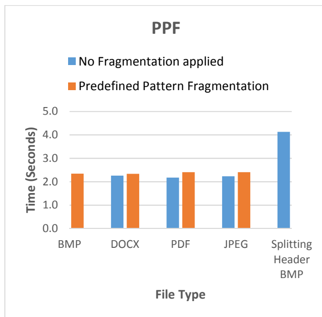
Figure 9 Predefined Pattern fragmentation results with a comparison of the same file without the technique applied
