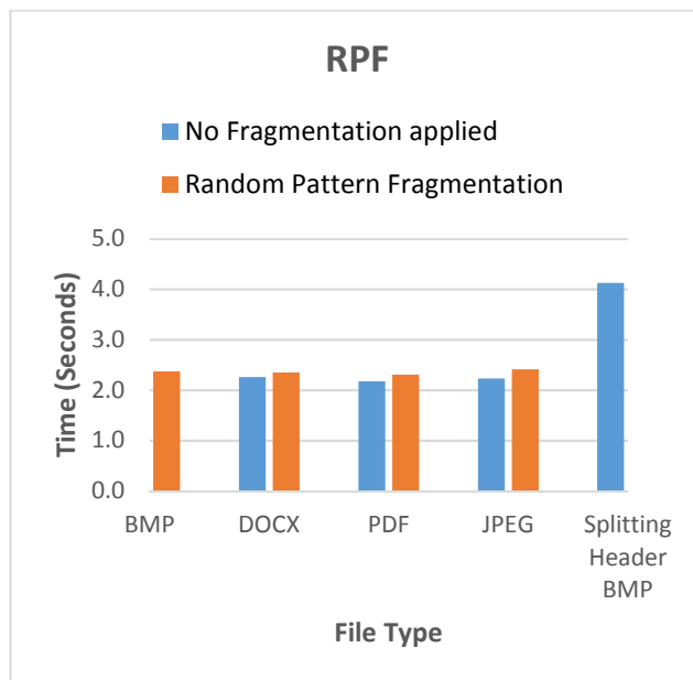
Figure 10 Random pattern fragmentation results with a comparison of the same file without the technique applied
