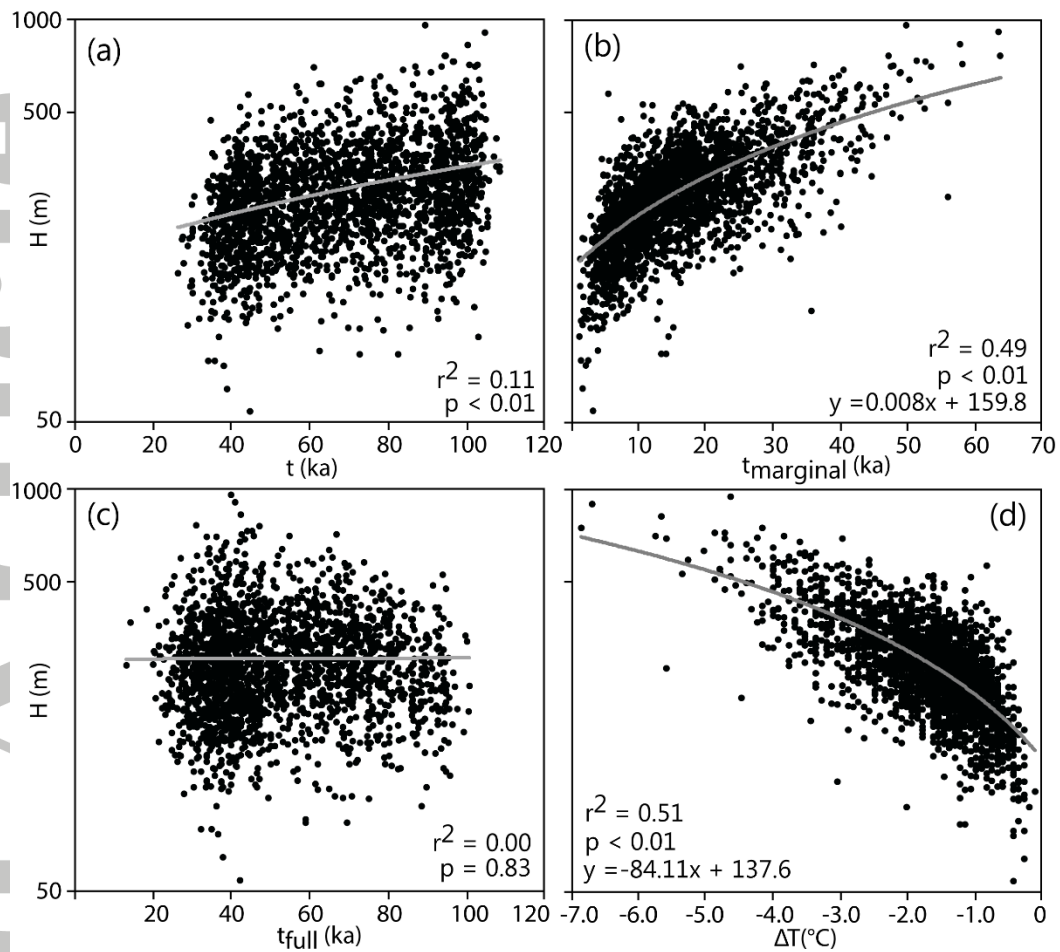
Fig. 6. Cirque depth ( H ) in Britain and Ireland plotted against the duration of the last glacial cycle (120 ka to present) that our modelling suggests they were (a) glacier-occupied ( t ); (b) occupied by small (largely cirque-confined) glaciers ( t_{\text{marginal}} ); and (c) occupied by large glaciers (which extended beyond cirque confines) ( t_{\text{full}} ). (d) H plotted against the \Delta T required for individual cirques to transition from A_c = 10\% to A_c = 90\% . Note: in all examples, the y-axes are plotted on logarithmic scales.
