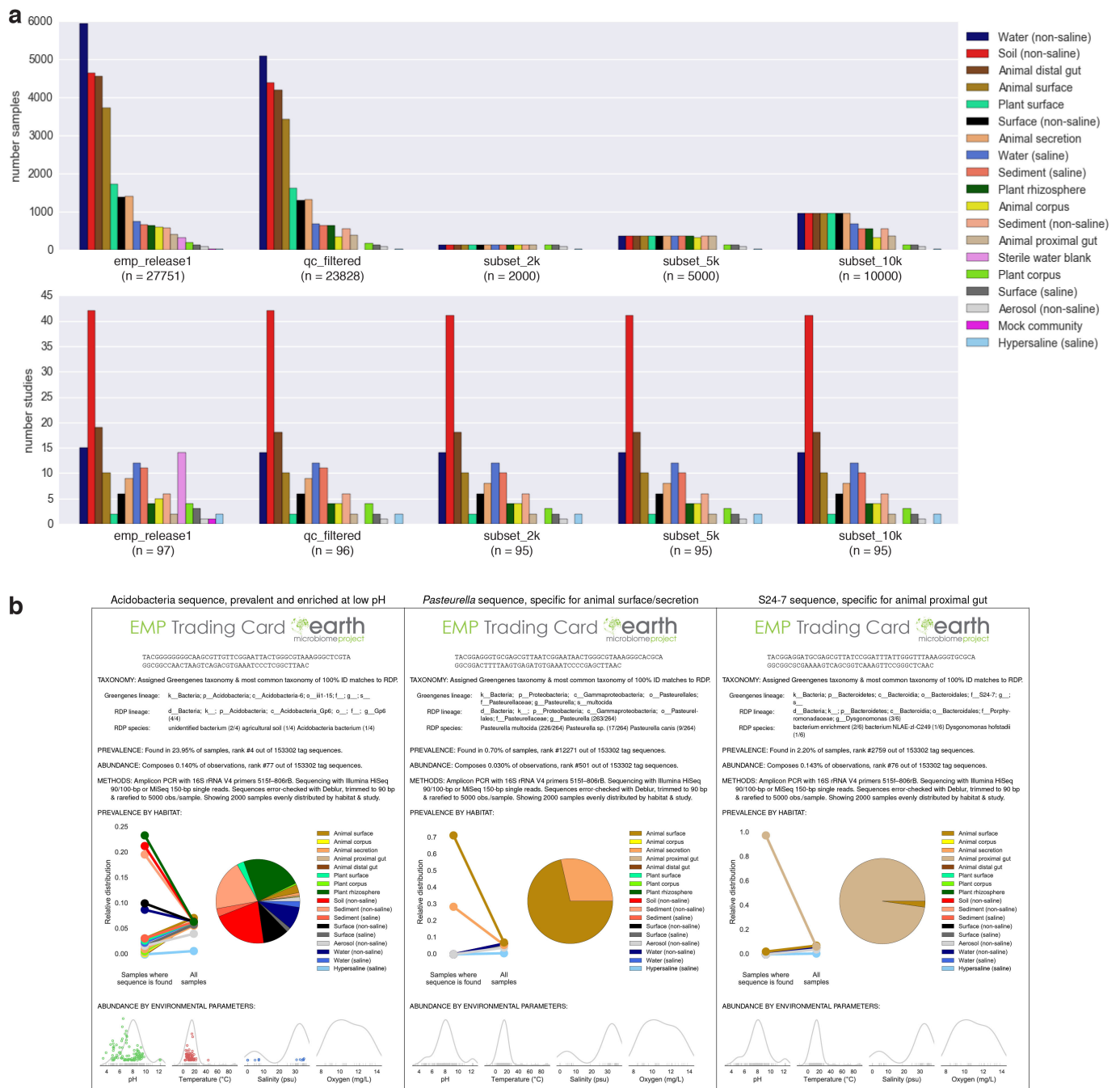
Extended Data Figure 7 | Subsets and EMP trading cards. a , Subsets of the EMP dataset with even distribution across samples and studies. Shown are all EMP samples included in this manuscript (release 1), the QC-filtered subset, and subsets of 10,000, 5,000, and 2,000 samples. The latter three contain progressively more even representation across environments and studies, providing a more representative view of the Earth microbiome and a more lightweight dataset. Top, histograms of samples per environment (EMPO level 3) for each subset. Bottom, histograms of studies per environment (EMPO level 3) for each subset. b , EMP trading cards: distribution of 16S rRNA tag sequences across the EMP. Trading cards highlight the power of the EMP dataset to help define niche ranges of individual microbial sequence types across the planet's microbial communities. Cards show distribution of 16S rRNA tag sequences in a 2,000-sample subset of the EMP (rarefied to 5,000 observations per sample) having even distribution by environment (EMPO level 3) and study. Taxonomy is from Greengenes 13.8 and Ribosomal Database Project (RDP), with the fraction of exact RDP matches by lineage and species name shown in parentheses. The pie chart and point plot show the
