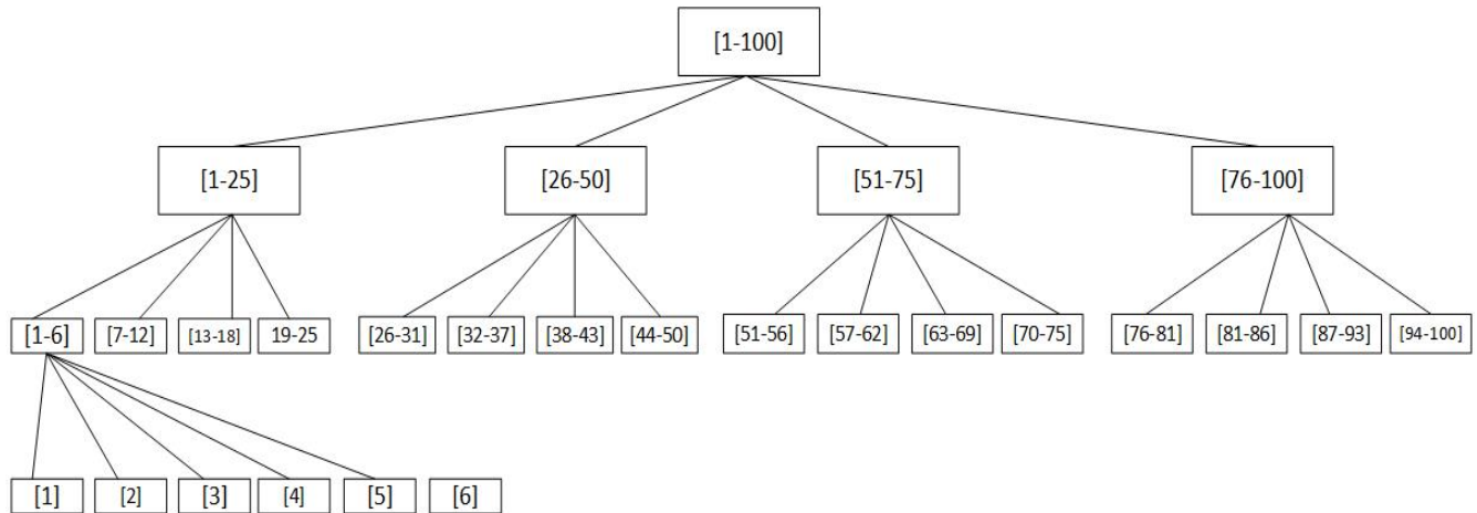
FIGURE 1. Generalization hierarchy.
