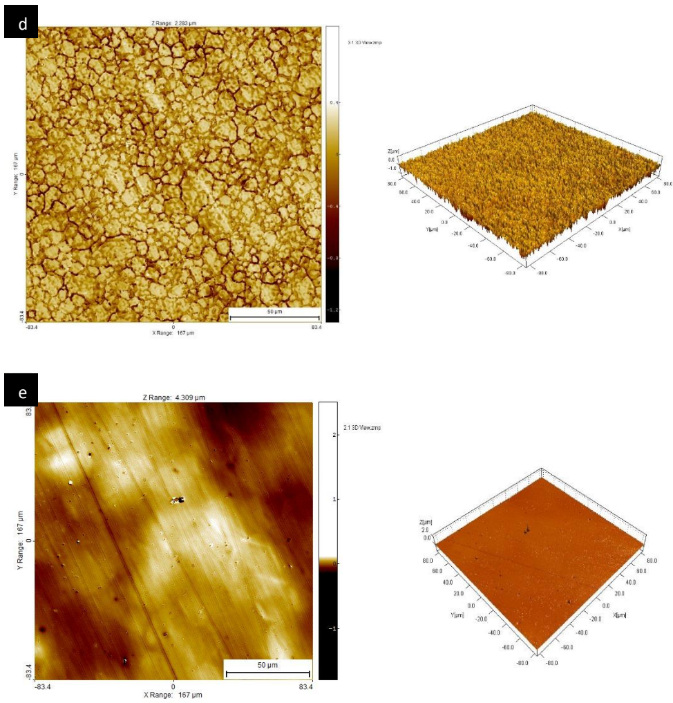
Figure 29 continued: White light profilometry pictures demonstrating the topography of the surfaces in 2D and 3D after retention assays of S. aureus with 10 % bovine plasma on d) 316TiN, and e) TiN/15.03at.%Ag surfaces.
