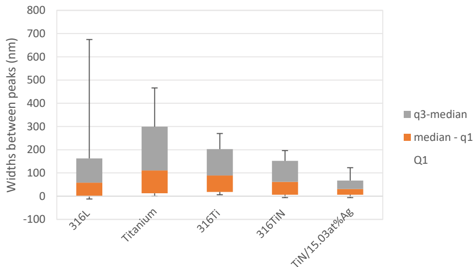
Figure 42: Distribution of peak widths obtained from white light profilometry line profiles demonstrating the distribution of peak width sizes between the 5 largest and 5 smallest widths between peaks from 3 different line profiles (n = 3).
