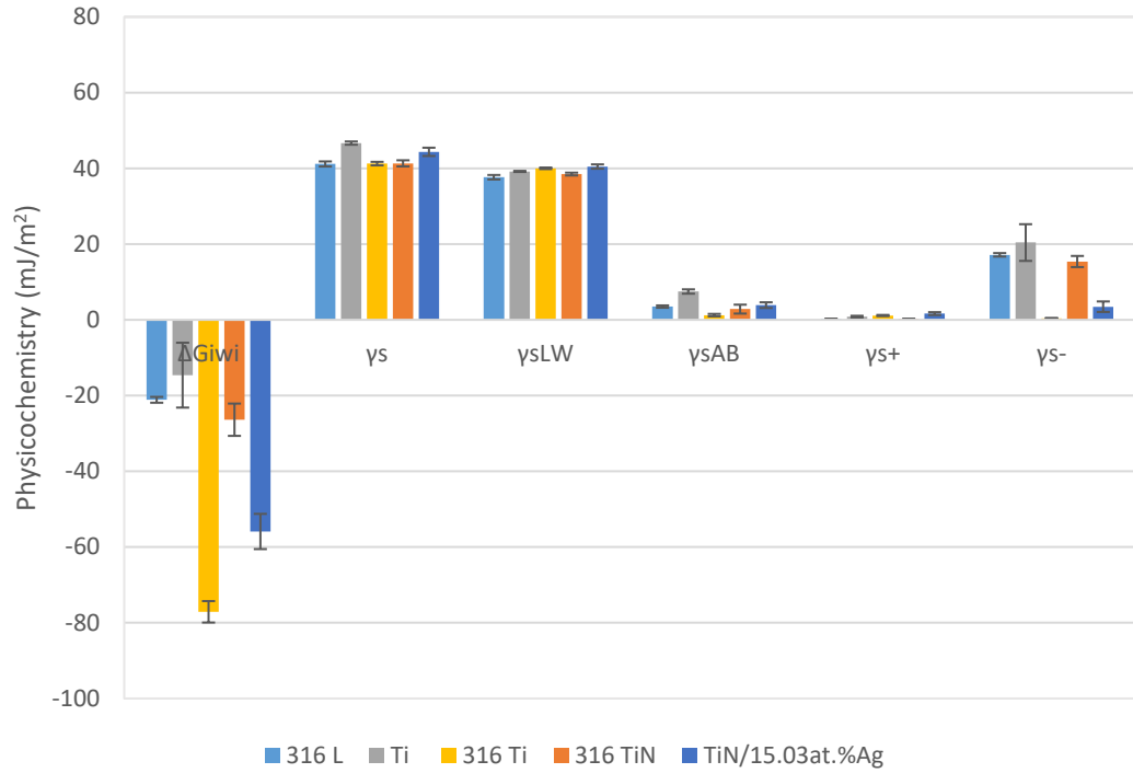
Figure 63: Physicochemistry of the metal surfaces once conditioned with E. coli \pm standard error (n = 3).
