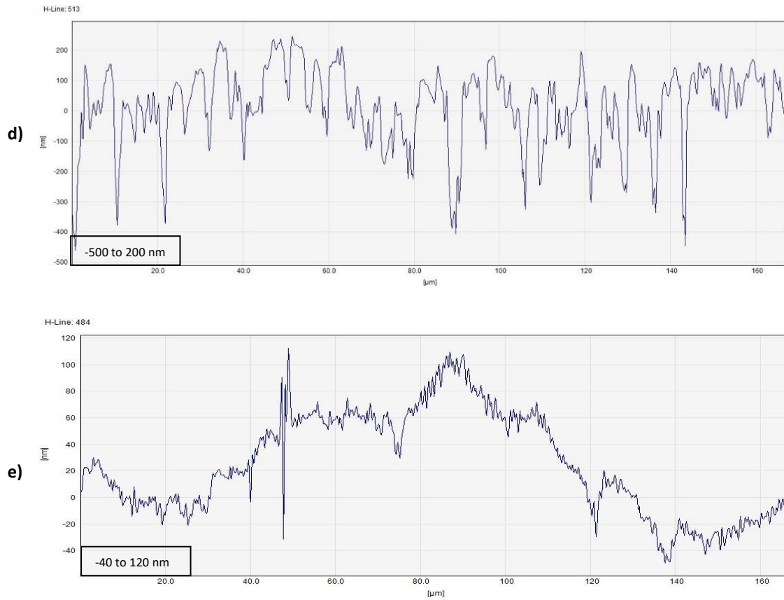
Figure 39 continued: d) 316TiN, and e) TiN/15.03at.%Ag surfaces demonstrating the micro and nano topographies of the 160 μm surfaces. Three areas of three coupons were analysed (n = 9). Note the changes to scale on the Y axis.
