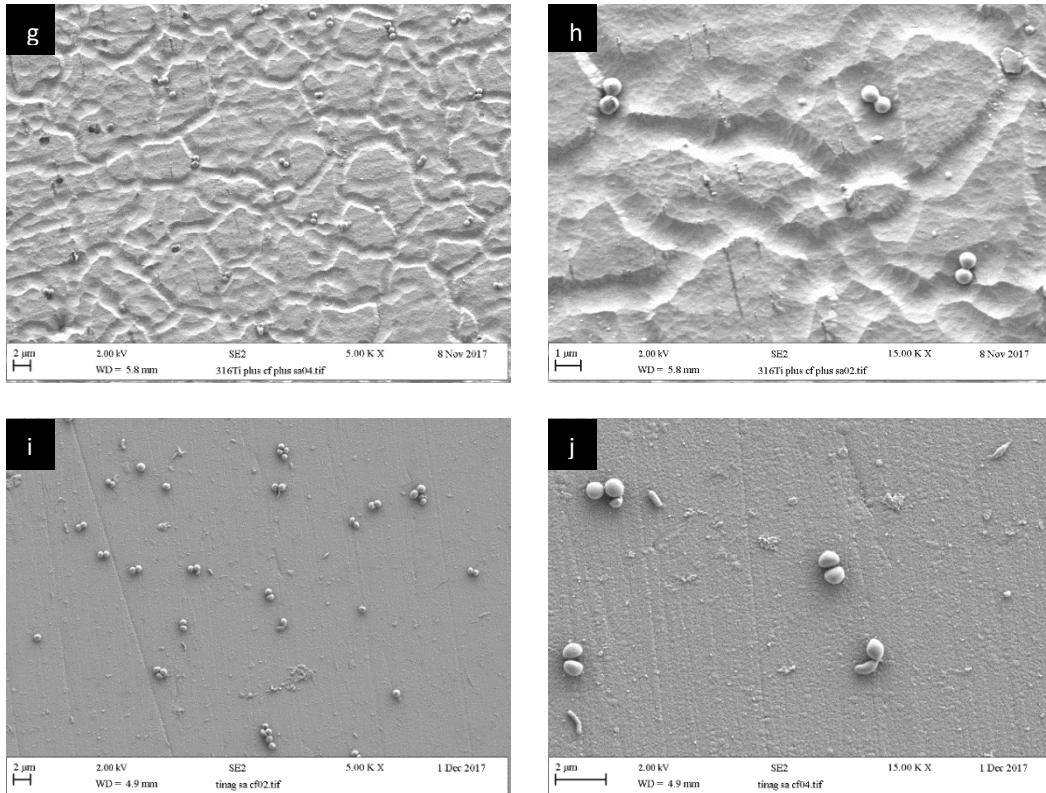
Figure 23 continued: g) 316TiN x 5,000 magnification, h) x 15,000 magnification, i) TiN/15.03at.%Ag x 5,000 magnification, j) x 15,000. Images allow qualitative assessment of the interaction between the S. aureus cells with the conditioning film and the macro and micro topographies of the different surfaces.
