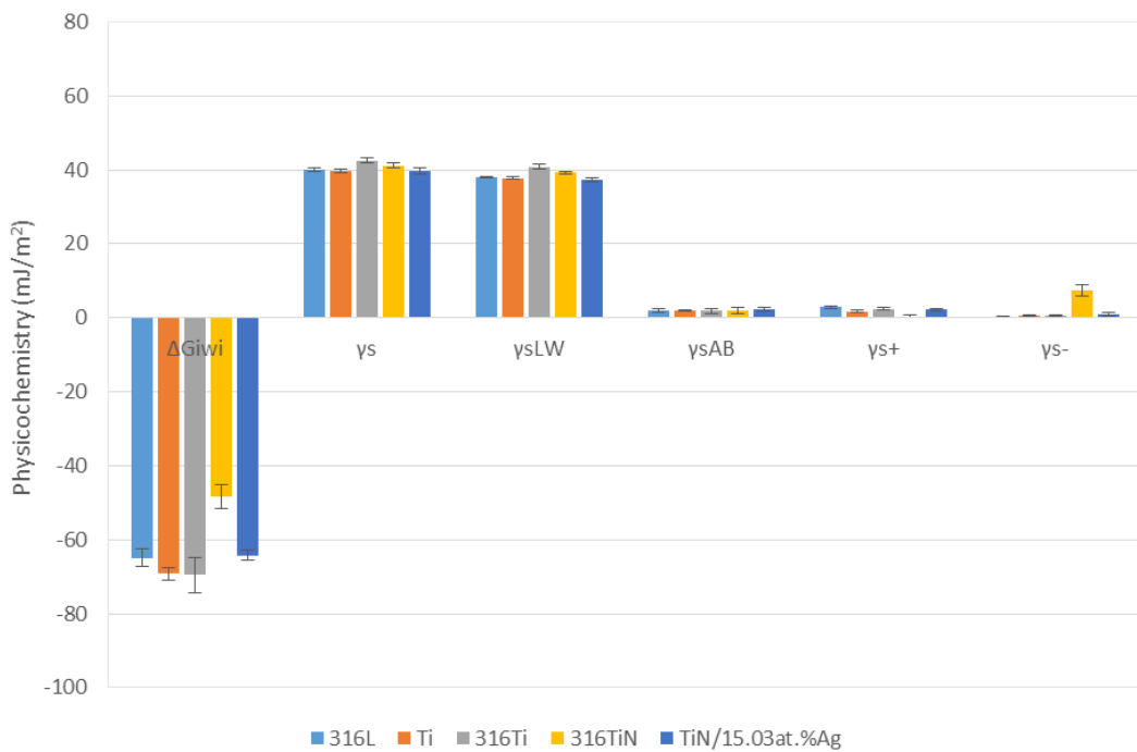
Figure 64: Physicochemical properties of the five metal surfaces post retention assay of 10 % bovine plasma \pm standard error (n = 3).
