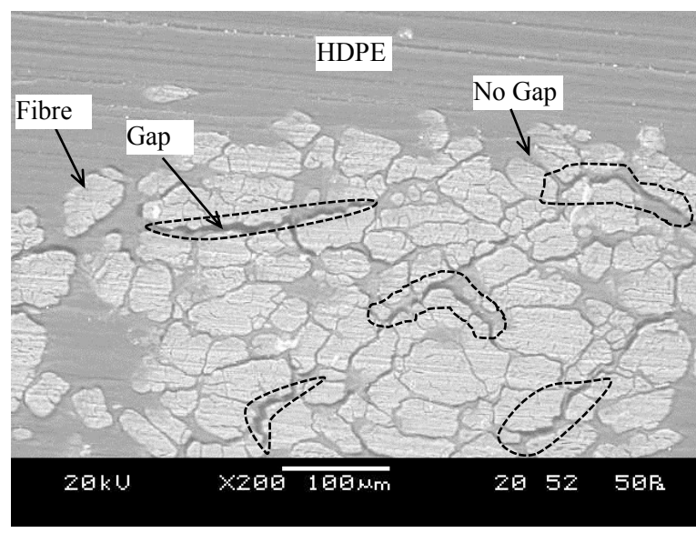
Fig. 7. Cross-sectional view of Jute yarn in HDPE matrix showing gaps between fibres and matrix
