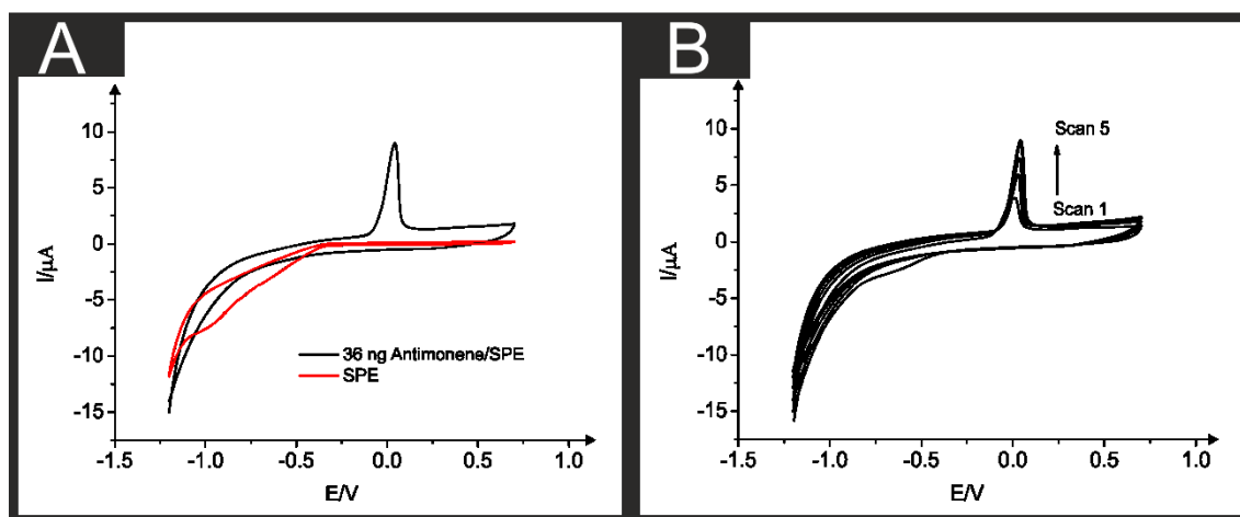
Figure S3. (A) Cyclic voltammograms of bare SPE (red) and 36 ng antimonene/SPE (black). (B) Successive cyclic voltammograms of 36 ng antimonene/SPE. In both cases CVs were obtained at 0.5 M H 2 SO 4 using a three electrodes system.
