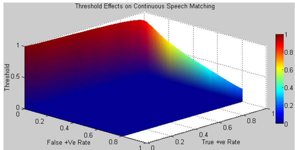
Fig. 7 Measuring the optimal threshold value for query and reference frames match/mismatch decision using ROC curve
