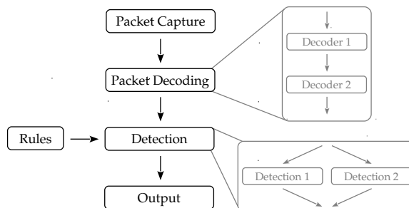
Fig. 6. Suricata architecture.
