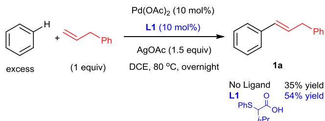
Scheme 1. S,O-Ligand promoted C–H olefination of benzene.
