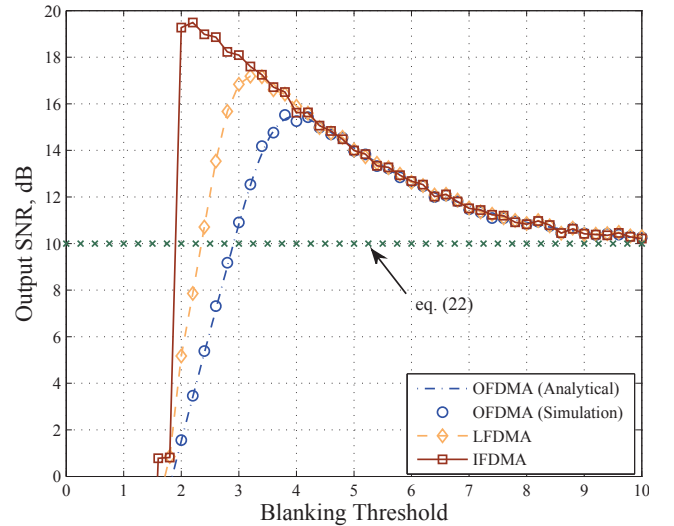
(a) Blanking.
