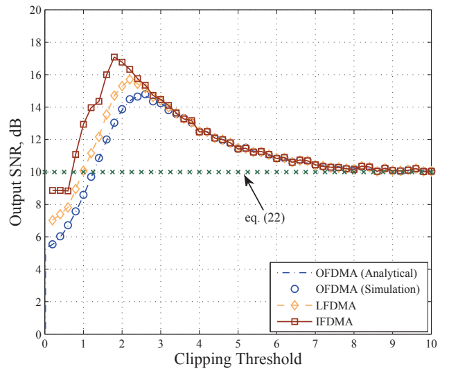
(b) Clipping.
